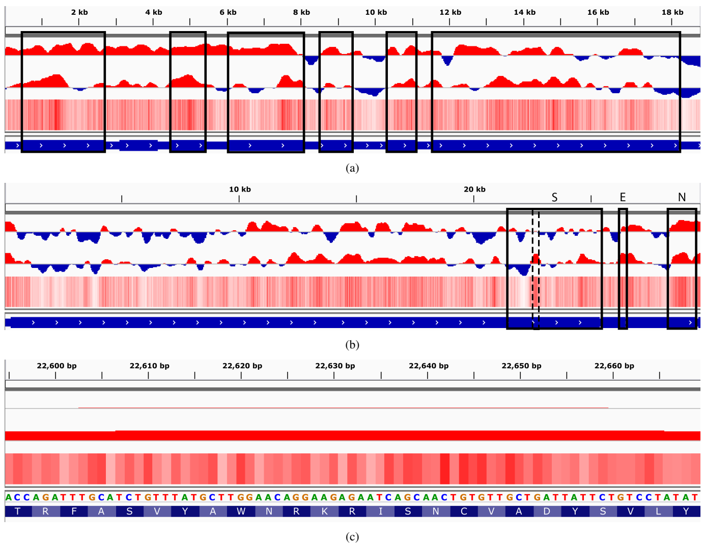
Figure 2. Taï Forest ebolavirus and SARS-CoV-2 coronavirus genomes. Top: score predicted by LSTM All . Middle: score predicted by CNN All . Heatmap: nucleotide contributions of CNN All . Bottom, in blue: reference sequence. 2a: Taï Forest ebolavirus. Genes that can be detected by at least one model are highlighted in black. 2b: Whole genome and sequences encoding the spike protein (S), envelope protein (E) and nucleocapsid protein (N). 2c: Spike protein gene, a small peak (positions 22,595-22,669, dashed line in Fig. 2b) within the receptor-binding domain (predicted by CD-search, positions 22,517-23,185). Binding to the receptor is crucial for entry to the host cell. Local host adaptation could help switch hosts between the animal reservoir and humans.
