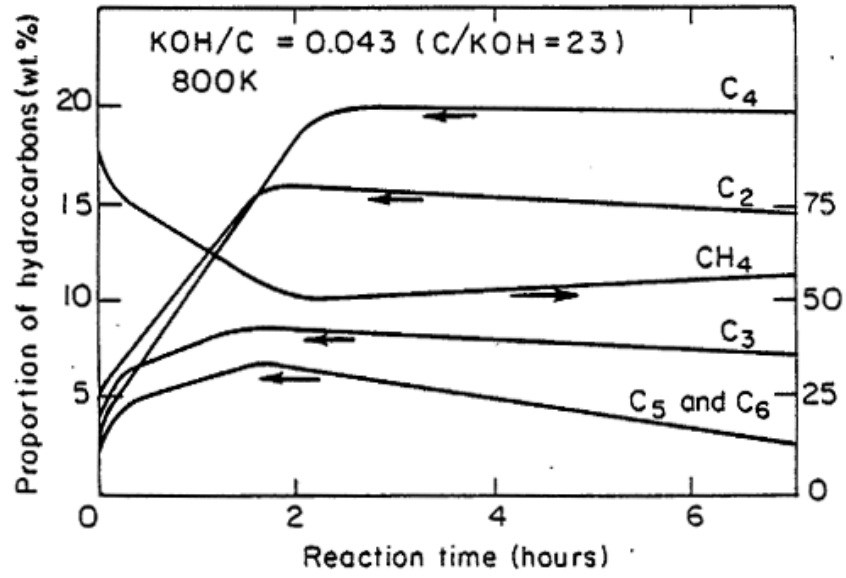
Figure 2 Plot of dependence on reaction time of the proportion of hydrocarbons for a KOH/C loading equal to 0.043 (mol).
