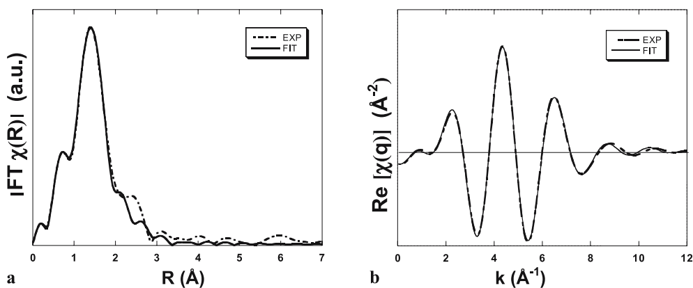
FIGURE 7 Cu-K edge moduli of Fourier transform (a) and best fit (b) for the green sample PM35117. Transformation was performed in the interval k = 3\text{--}10 \text{ \AA}^{-1} with a k^1 -weight
