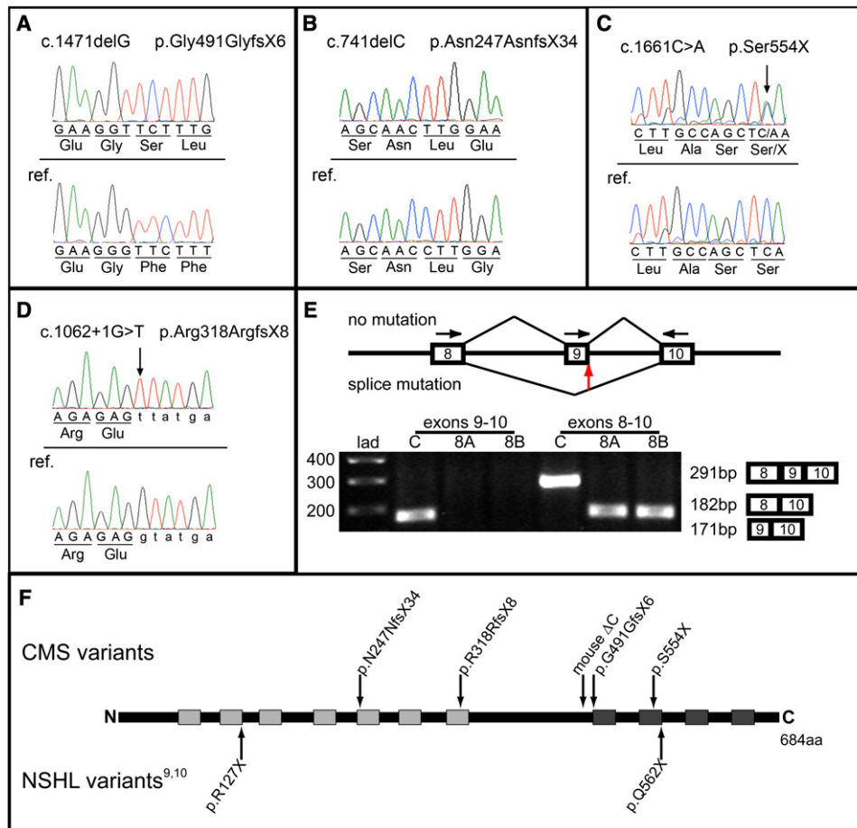
Figure 2. GPSM2 Sequence Analysis and GPSM2 Schematic
