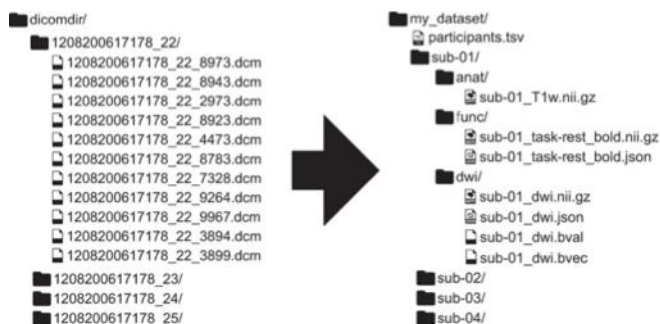
Figure 1. Transformation between DICOM and BIDS 3 .
