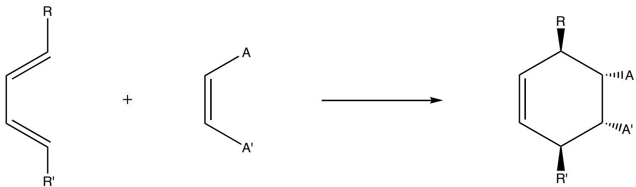
Figure 1: The Diels-Alder Reaction. The R's stand for a generic substituent and the A's stand for an electron accepting substituent. Adapted from (Vollhardt et. al., 1994, p. 540).
