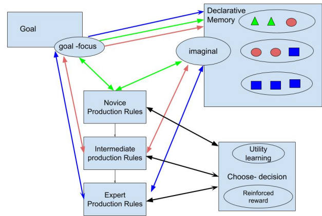
Figure 3: Level of expertise mechanism in VSM-ACTR.
