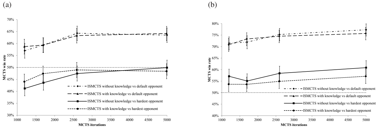
Figure 1: Playing strength of MCTS AI versus knowledge-based AI, for (a) the standard game of Spades; (b) the modified game where every round features a nil bid. Error bars show 95% confidence intervals.
