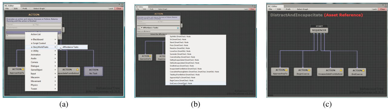
Figure 5: Parameterized Behavior Tree Design. (a) Select an affordance task to add to an action node. (b) Select an affordance to use in the behavior tree. (c) Graph of created behavior tree.
