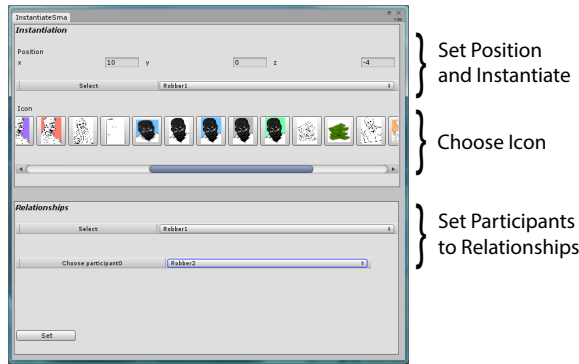
Figure 4: Smart Object Instantiation. Instantiate a smart object by defining position and a representative icon. Set the participants to the relationships.
