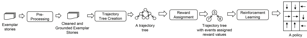
Figure 1: The Quixote system workflow.
