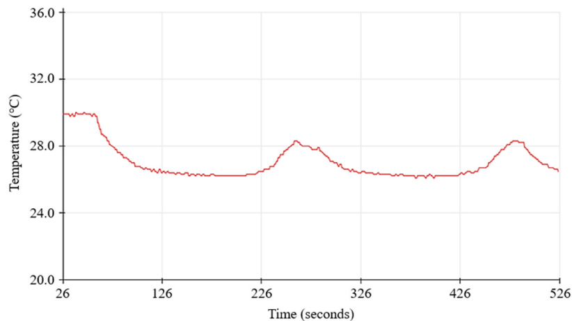
(b) Temperature regulation curve–cooling cycle
