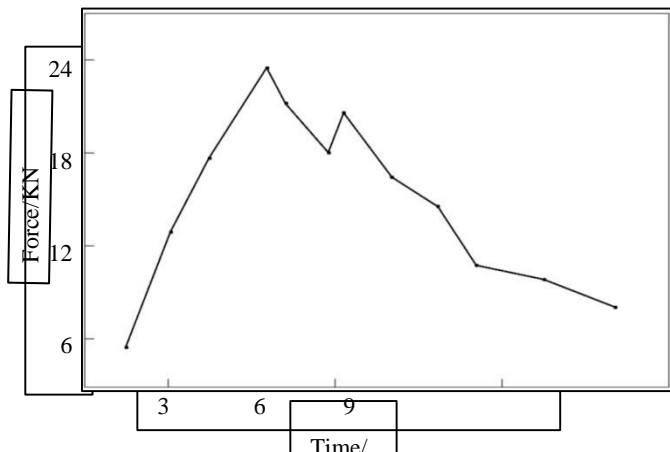
Figure 12: Bucket forces during the pick-up phase
