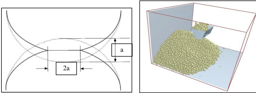
Figure 1: Particle contact deformation diagram Figure 2: Shovel loading simulation
