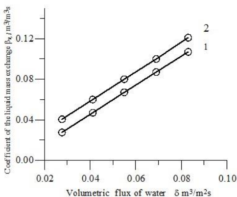
Fig. 3. Coefficient of the liquid mass exchange \beta_{v,l} versus volumetric flux of water \beta , 1- u= 10 m/s, 2- u= 20 m/s.
