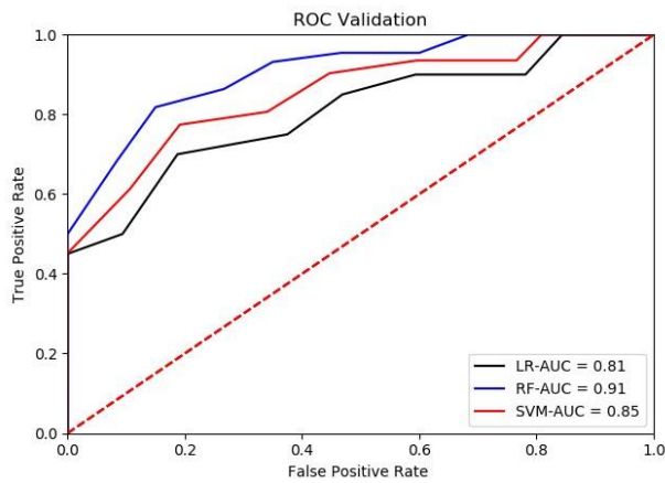
(b) ROC curve test results of each model after screening factors
