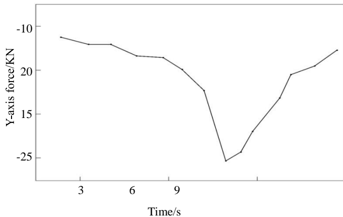
Figure 9: The Y-directional component of the digging resistance
