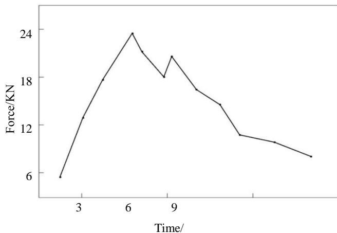
Figure 11: Bucket forces in the horizontal insertion phase
