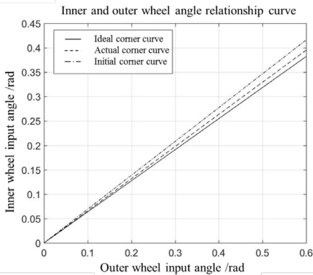
Figure.5 Inner and outer wheel angle relationship curve
