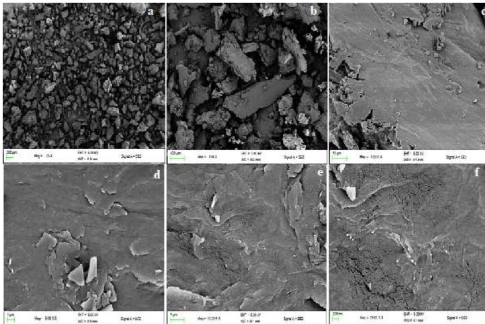
Figure 11. SEM micrographs for 25% RHA-MA-g-HDPE a. magnification at 25 X b. magnification at 100 X c. magnification at 1000 X d. magnification at 5000 X e. magnification at 10000 X f. magnification at 20000 X.
