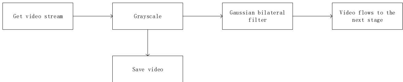
Figure 3. Preprocessing process
