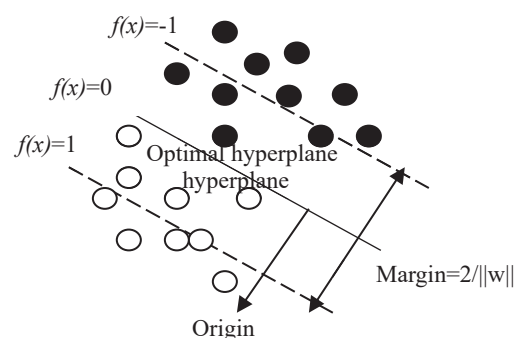
Figure 1. Optimal classifying line under linear classified condition
