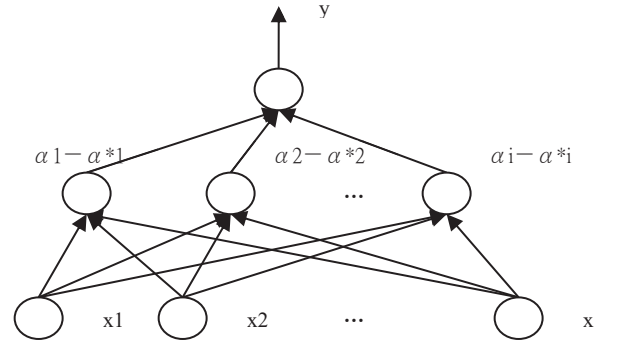
Figure 2. SVM network structure diagram
