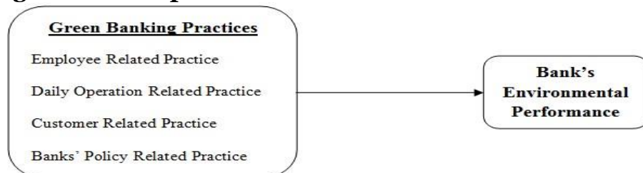
Figure 1: Conceptual Model
