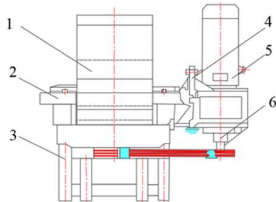
1. Feeding funnel; 2. Host device; 3. Host bracket; 4. Power bracket; 5. Power source; 6. Belt wheel
