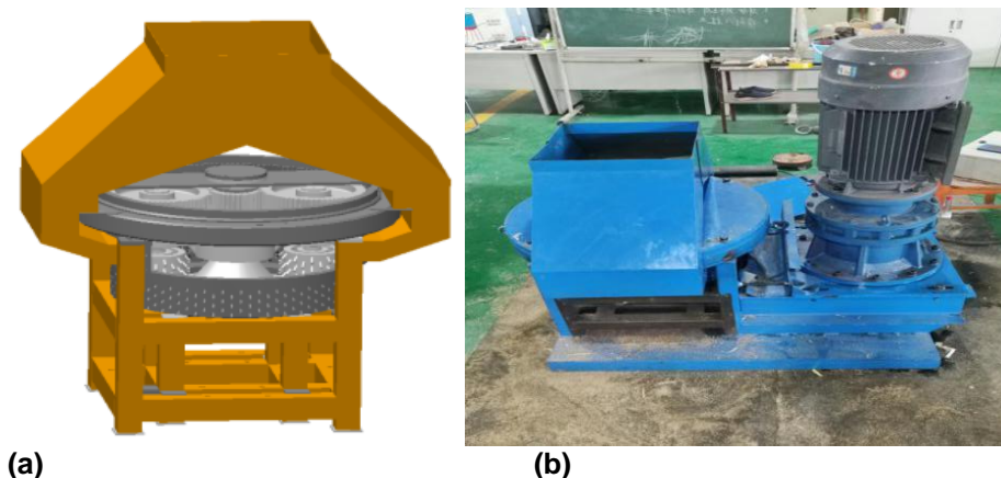
Fig. 6. Ring molding machine diagram
