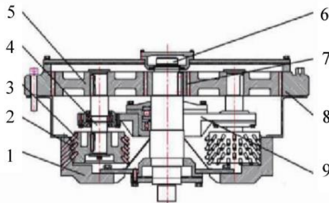
1. Ring mold body; 2. Compression cam; 3. Pressure roller body; 4. Pressure roller shaft; 5. Pressure roller shaft gear; 6. Spindle; 7. Spindle gear; 8. Straight-toothed cylindrical internal gear; 9. Coupling seat
