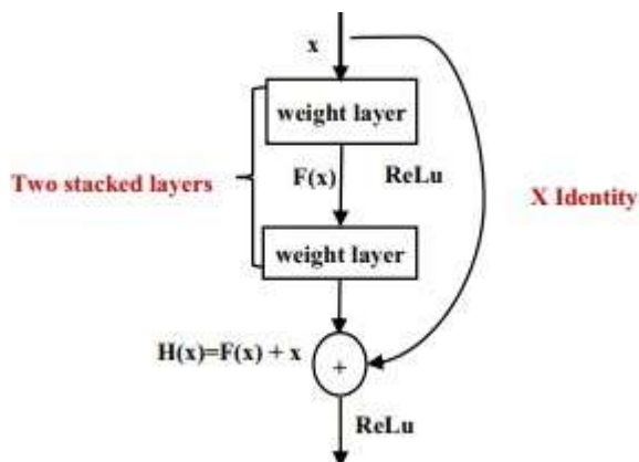
Figure4. Residual Network: a building block.
