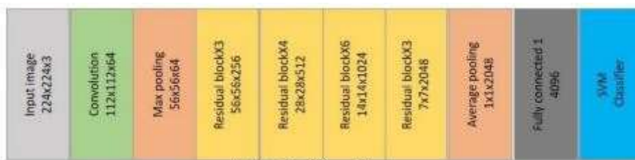
Figure 5. ResNet50 architecture
