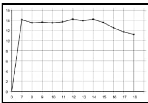
Figure 8 Experimental voltage of the PV panel
