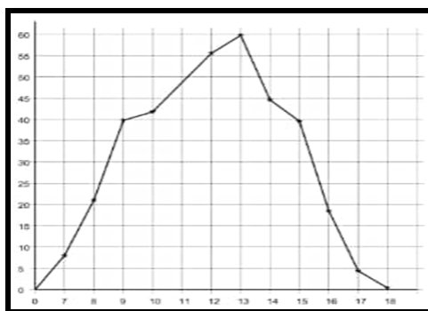
Figure 9 Experimental current of the PV Panel
