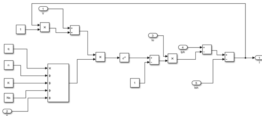
Figure 2 Simulink/Matlab block diagram of output current.
