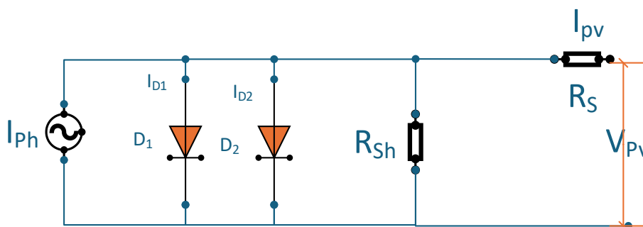
Figure 1 Illustration of conceptual circuit diagram of two-diode model
