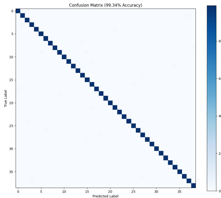
Figure 2 Confusion Matrix
