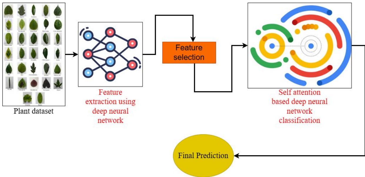
Figure 1 Methodology Flowchart
