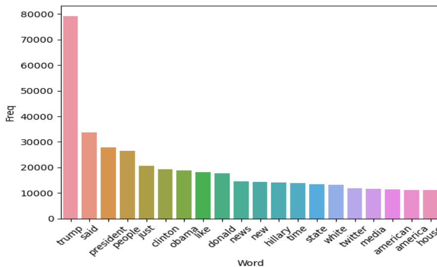
Fig. 3. This bar chart displays the most prevalent words in the dataset along with the frequencies that correspond to them. Donald Trump is associated with a significant portion of the dataset, as evidenced by the fact that the word "Trump" appears far more frequently than any other word. This might indicate that the dataset contains a large number of news items, discussions, or debates about Trump, possibly related to politics or elections. Words like "said," "president," "people," and "just" are also commonly used. These are general terms that are commonly used in news reporting, even though "said" is often used to quote statements.
