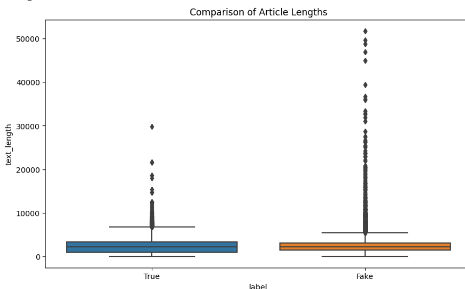
Fig. 2. The relatively close median (middle line in each box) for each type of news indicates that the normal lengths of fake and true news stories are similar. The box displays the IQR, or middle 50% of the data. The somewhat larger IQR for True news articles compared to Fake articles suggests that True news articles typically have more variance in duration.
