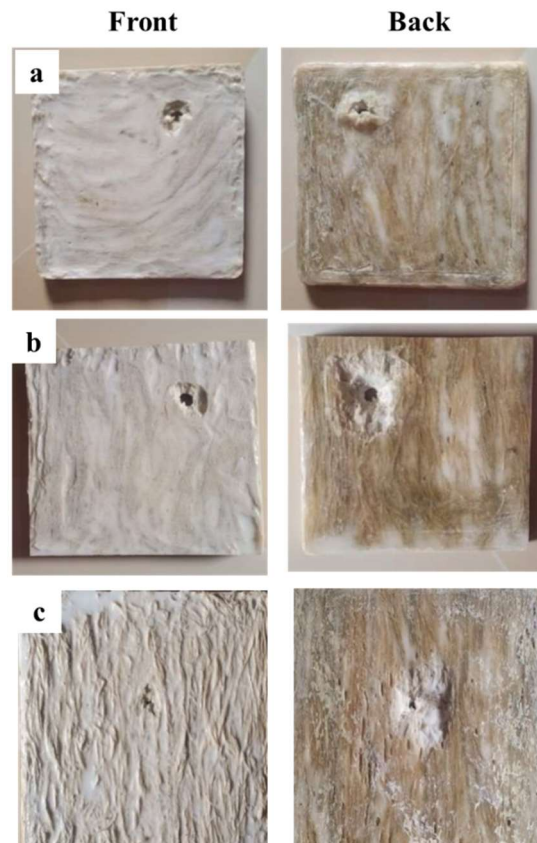
Figure 1. Ballistic Testing Results (a) 10mm Thickness (b) 15mm Thickness (c) 20mm Thickness [5]
