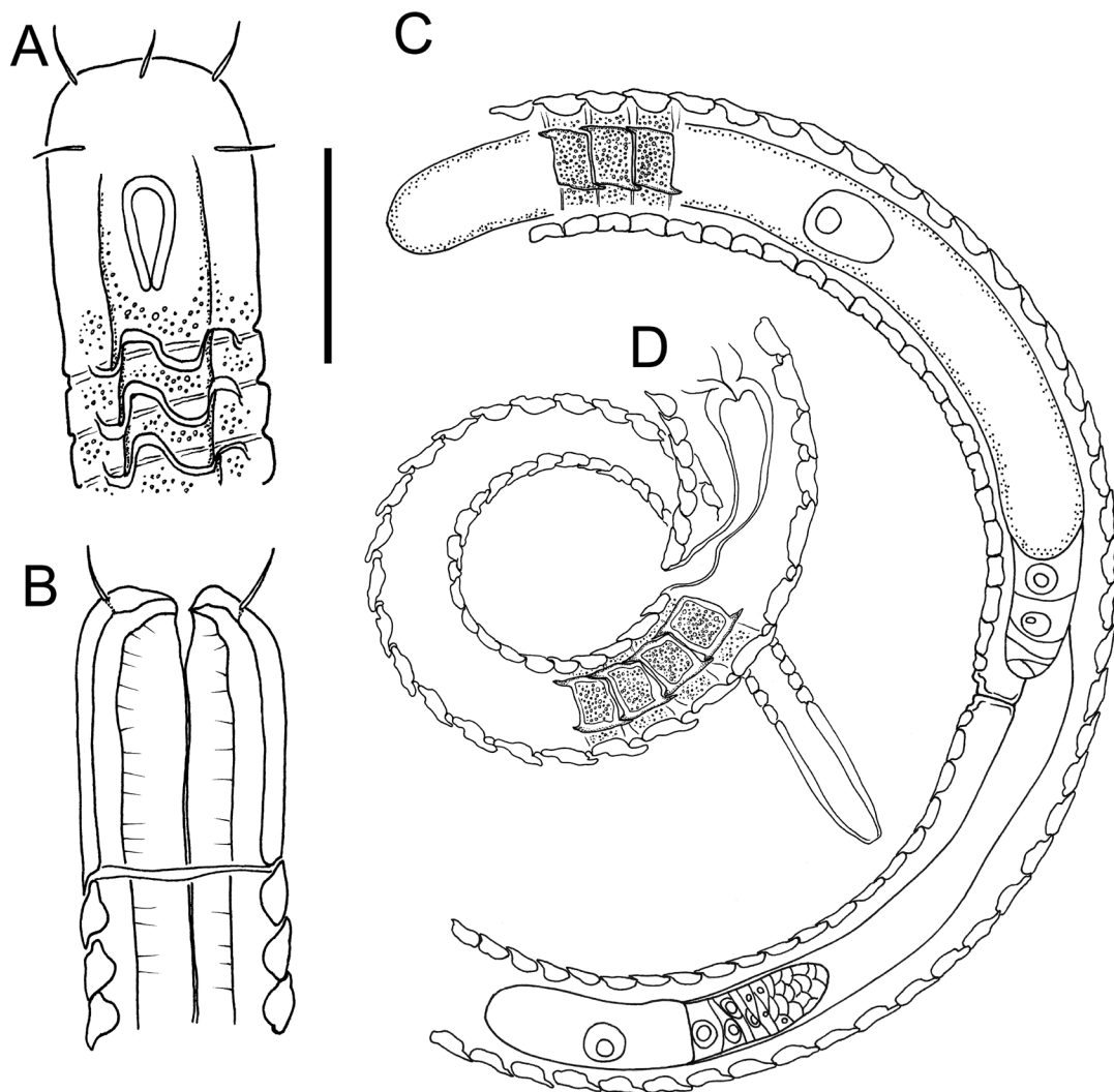
Fig. 3. Ceramonema taikoraha sp. nov., paratype, ♀ (NIWA 154944). A. Surface view of cephalic region. B. Optical section of cephalic region. C. Reproductive system. D. Posterior body region. Scale bar: A–B = 30 \mu\text{m} ; C = 47 \mu\text{m} ; D = 37 \mu\text{m} .
