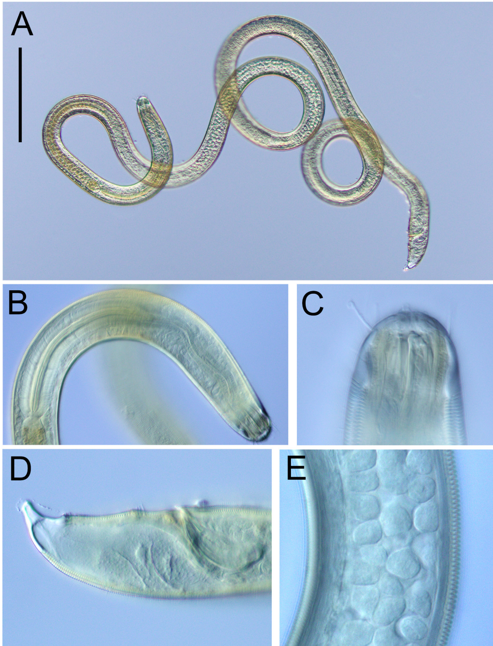
Fig. 13. Acanthopharynx dormitata Leduc & Zhao, 2016, ♂ (NIWA 154953). A. Entire body. B. Pharyngeal region. C. Cephalic region and buccal cavity. D. Cloacal and tail region. E. Sperm. Scale bar: A = 200 µm; B = 85 µm; C = 22 µm; D = 44 µm; E = 26 µm.
