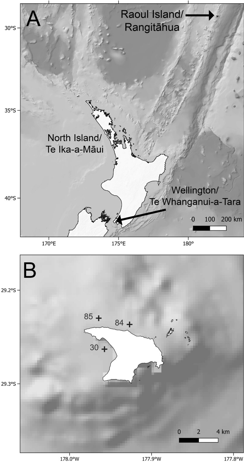
Fig. 1. Map showing locations. A. Raoul Island and Wellington city at southern end of New Zealand's North Island (northern portion of South Island also visible). B. Subtidal sampling sites off the coast of Raoul Island identified by their station numbers.
