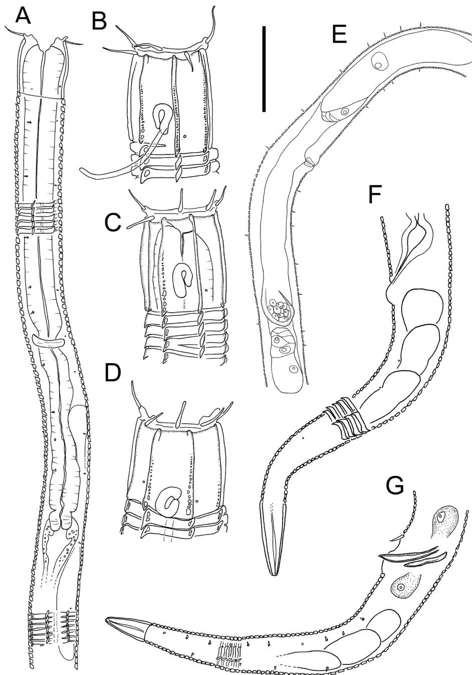
Fig. 7. Metadasynemoides taihua sp. nov. A, G. Holotype, ♂ (NIWA 154947). B–F. Paratypes (NIWA 154948). A. Pharyngeal body region. B. ♂, cephalic region. C. ♀, cephalic region. D. ♀, cephalic region. E. ♀, reproductive system. F. ♀, posterior body region. G. Posterior body region. Scale bar: A = 50 \mu\text{m} ; B–D = 30 \mu\text{m} ; E = 67 \mu\text{m} ; F–G = 40 \mu\text{m} .
