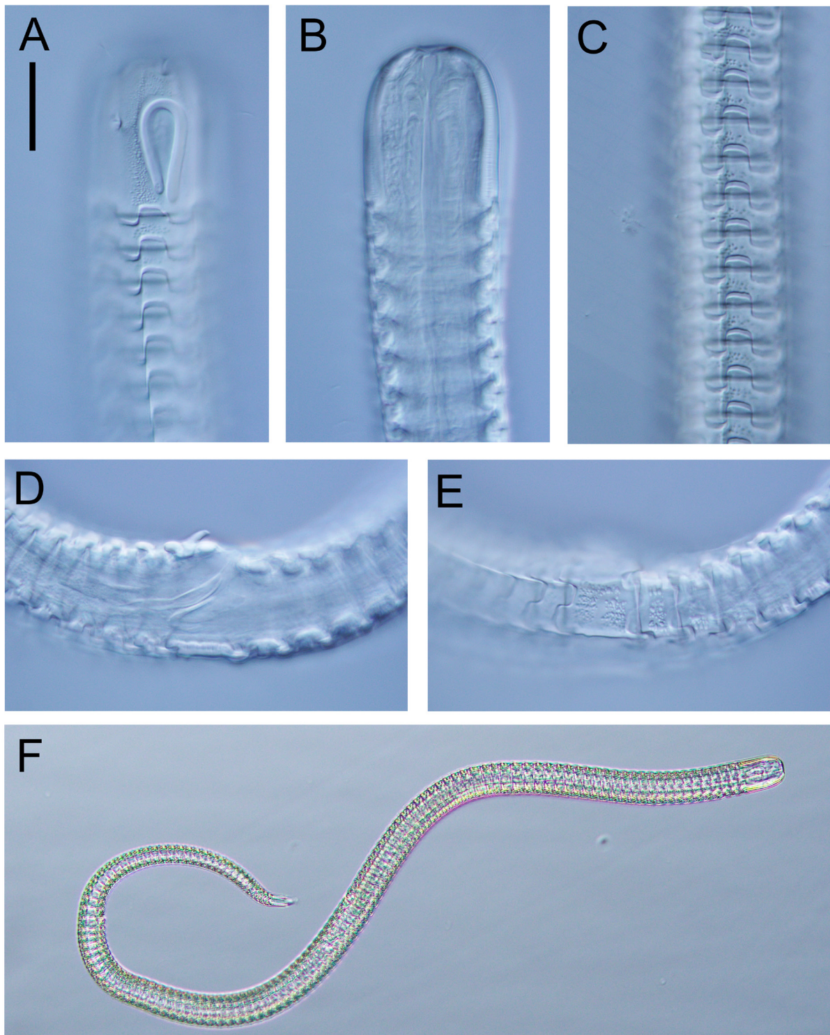
Fig. 6. Ceramonema taiora sp. nov., paratypes (NIWA 154946), light micrographs. A. ♂, surface view of cephalic region. B. ♂, optical section of cephalic region. C. ♂, surface view of cuticle, mid-body region. D. ♂, cloacal region, showing specular apparatus and precloacal spine. E. ♂, surface view of cloacal region. F. Entire female. Scale bar: A–E = 20 \mu m; F = 85 \mu m.
