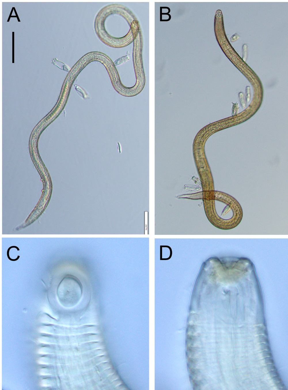
Fig. 14. Desmodora bilacinia Leduc & Zhao, 2016 (NIWA 154954). A. Entire male. B. Entire female. C. ♂, cephalic region showing amphidial fovea. D. ♂, cephalic region showing buccal cavity. Scale bar: A–B = 100 \mu m; C–D = 11 \mu m.
