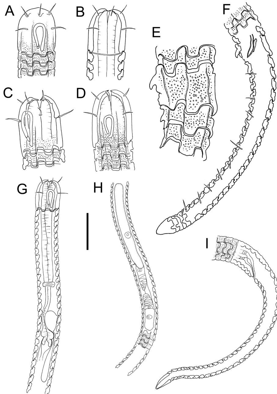
Fig. 5. Ceramonema taiora sp. nov. A–B, G. Holotype, ♂ (NIWA 154945). C–F, H–I. Paratypes (NIWA 154946). A. Cephalic region, surface view. B. Cephalic region, optical cross-section view. C. ♂, cephalic region, combined (super-imposed) surface and cross-section views. D. ♀, cephalic region, view. E. ♂, cloacal region. F. ♂, posterior body region. G. Pharyngeal body region. H. ♀, reproductive system. I. ♀, posterior body region. Scale bar: A–D = 30 µm; E = 16 µm; F = 33 µm; G, I = 45 µm; H = 68 µm.
