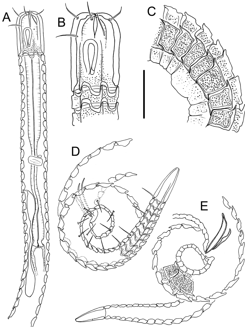
Fig. 2. Ceramonema taikoraha sp. nov., ♂♂. A–C, E. Holotype (NIWA 154943). C. Paratype (NIWA 154944). A. Pharyngeal region. B. Cephalic region. C. Surface of cloacal region. D. Posterior body region. E. Posterior body region showing copulatory apparatus. Scale bar: A = 45 \mu\text{m} ; B = 25 \mu\text{m} ; C = 18 \mu\text{m} ; D–E = 27 \mu\text{m} .
