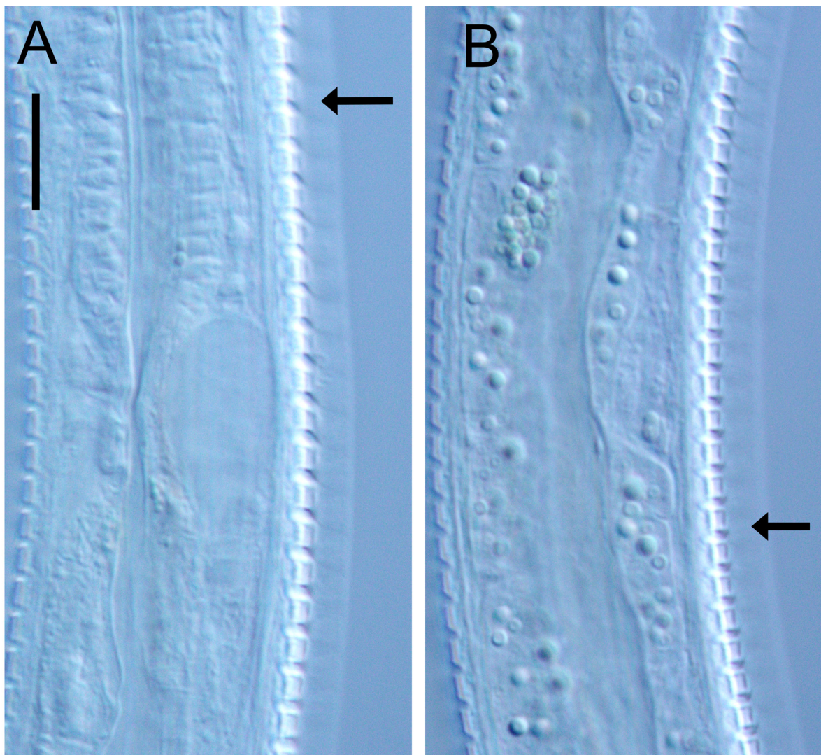
Fig. 9. Metadasynemoides taihua sp. nov., holotype, ♂ (NIWA 154947), light micrographs. A. Pharyngeal body region at level of secretory-excretory system (ampulla). B. Mid-body region. Arrows show membrane extending from body annule epicristae. Scale bar = 10 \mu\text{m} .
