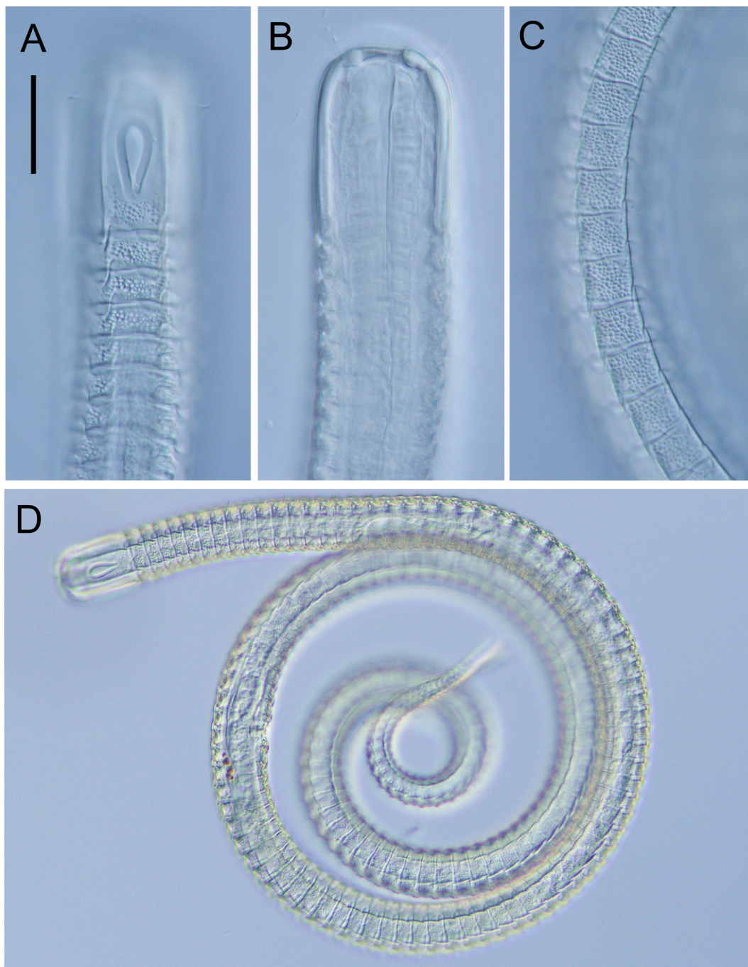
Fig. 4. Ceramonema taikoraha sp. nov., paratypes (NIWA 154944), light micrographs. A. ♀, surface view of anterior body region. B. ♀, optical section of anterior body region. C. ♂, surface view of cuticle. D. Entire female. Scale bar: A–C = 20 µm; D = 50 µm.
