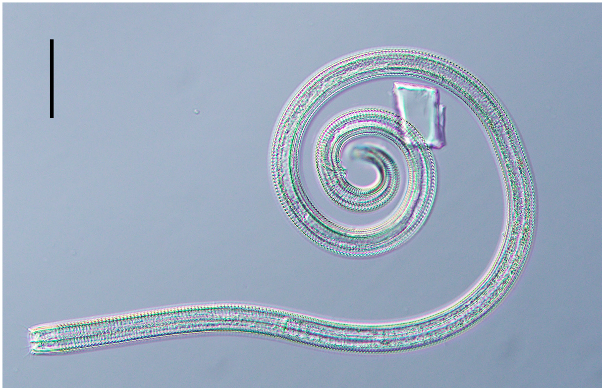
Fig. 10. Metadasynemoides taihua sp. nov., paratype, ♂ (NIWA 154948), light micrograph. Scale bar = 75 \mu\text{m} .
