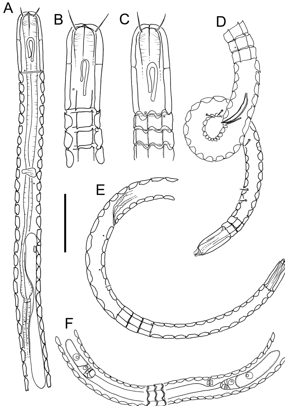
Fig. 11. Pselionema huakita sp. nov. A. Holotype, ♂ (NIWA 154949). B–F. Paratypes (NIWA 154950–1). A. Pharyngeal body region. B. ♀, cephalic region. C. ♂, cephalic region. D. ♂, posterior body region. E. ♀, posterior body region. F. ♀, reproductive system. Scale bar: A = 40 µm; B–C = 30 µm; D = 37 µm; E = 44; F = 52 µm.
