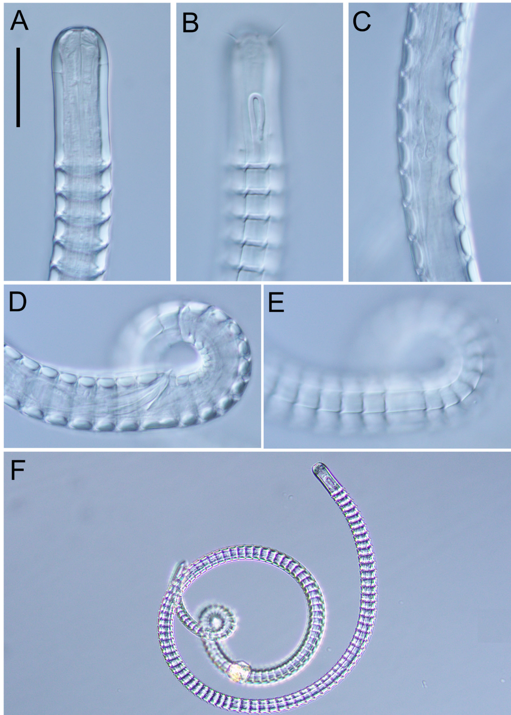
Fig. 12. Pselionema huakita sp. nov., light micrographs. A–B. Holotype, ♂ (NIWA 154949). C–F. Paratype, ♂ (NIWA 154950). A. Optical section of cephalic region. B. Surface view of cephalic region. C. Optical section showing junction of pharynx and intestine. D. Optical section of cloacal region. E. Surface view of cloacal region. F. Entire male. Scale bar: A–E = 40 \mu\text{m} ; F = 85 \mu\text{m} .
