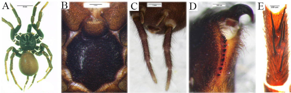
Fig. 8. Vacrothele baiseensis sp. nov., holotype, ♂ (DUIER, GX-VA-20231104001). A. Dorsal view. B. Maxilla, labium and sigilla. C. Spinnerets, right retrolateral view. D. Chelicera. E. Left leg II.
