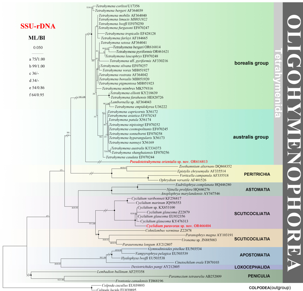
Fig. 6. The maximum likelihood tree inferred from the SSU-475 rDNA gene sequences, showing the positions of Pseudotetrahymena orientalis gen. et sp. nov. and Cyclidium paravorax sp. nov. (in red). Numbers at nodes represent the bootstrap values of maximum likelihood out of 1000 replicates and the inference. Fully supported (100%/1.00) branches are marked with solid circles. The scale bar corresponds to five substitutions per 100 nucleotide positions.
