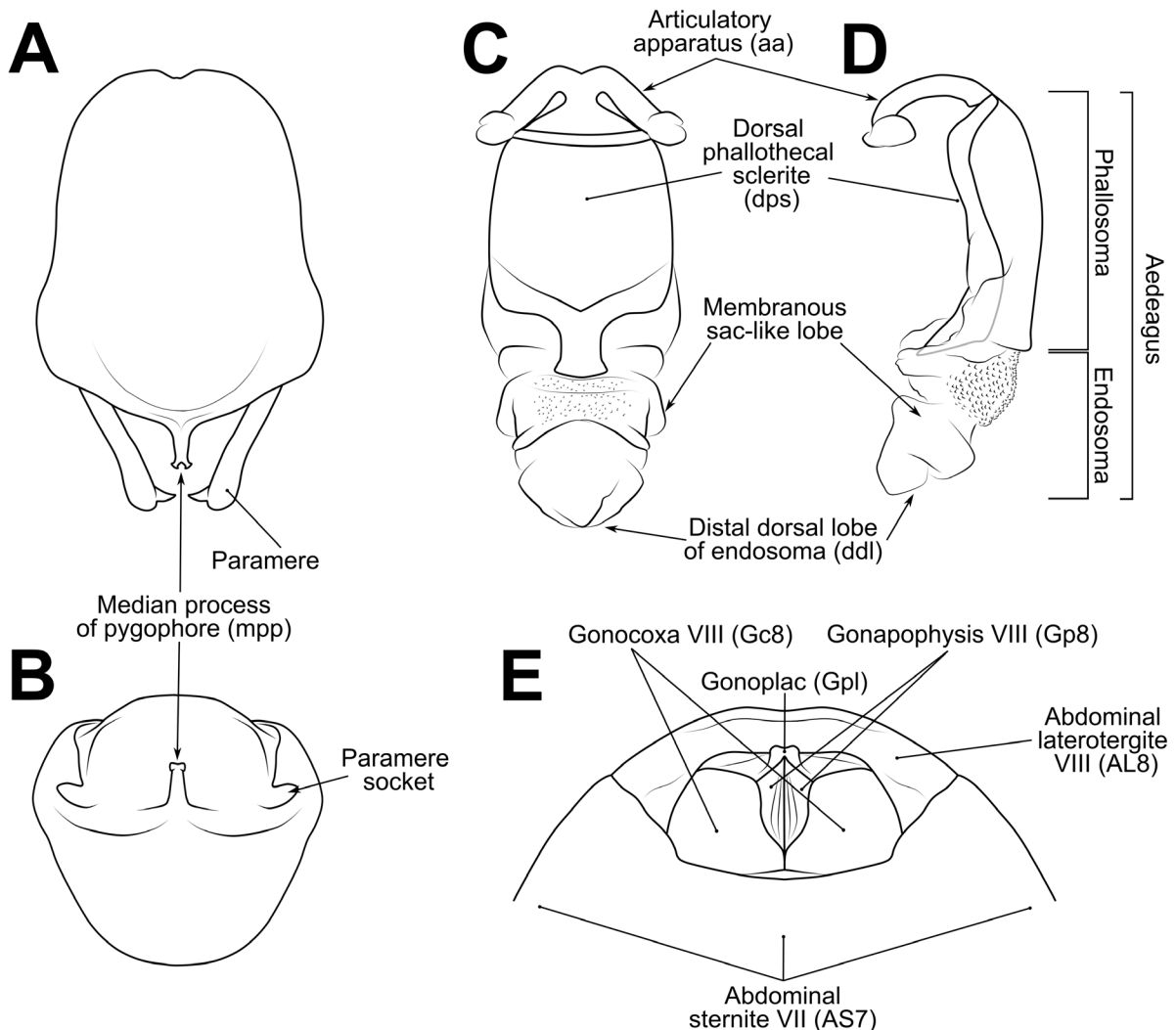
Fig. 2. Structure and morphological terms of species of Epidaus Stål, 1859 (cont.). Drawing based on Epidaus batxatensis Truong, Nguyen & Ha sp. nov. A–D. Holotype, ♂ (HNL2024-234). E. Paratype, ♀ (HNL2024-276). A. Pygophore with paramere of male genitalia in ventral view. B. Pygophore in caudal view. C. Phallus in dorsal view. D. Phallus in lateral view. E. Female external genitalia in ventral view.
