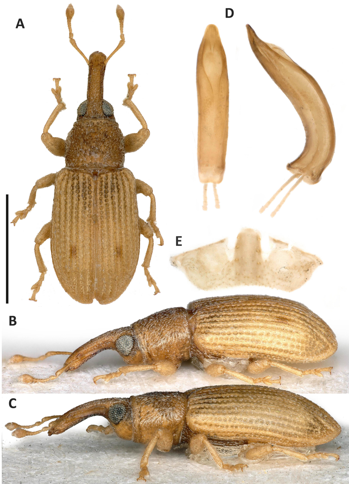
Fig. 7. Habitus of Derelomus lindbergi Roudier, 1957. A–B, D–E. Holotype, ♂ (Republic of Cabo Verde) (MZH). C. Paratype, ♀ (same locality) (MZH). A. Habitus in dorsal view. B–C. Habitus in lateral view. D. Penis in dorsal (left) and lateral (right) views. E. Stridulatory plate. Scale bar: 1 mm; D–E not to scale.
