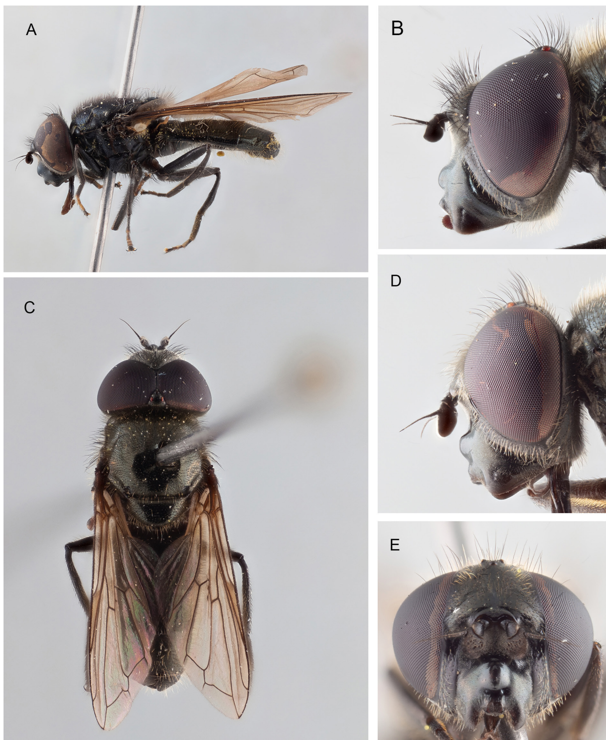
Fig. 10. Cheilosia ( Taeniochilosia ) bakurianiensis Kuznetzov, 1987. A. ♂ (FMT); habitus, lateral view; collected in Georgia; body length 7.0 mm. B. ♂ (FMT); head, lateral view; collected in Georgia; eye width 1.1 mm. C. ♂ (FMT); collected in Georgia; habitus, dorsal view; collected in Georgia; body length 7.3 mm. D. ♀ (FMT); head, lateral view; collected in Georgia; eye width 1.0 mm. E. ♀ (ZFMK, ZFMK-DIP-00093761); head, frontal view; collected in Armenia; facial width 2.1 mm. Not to scale.
