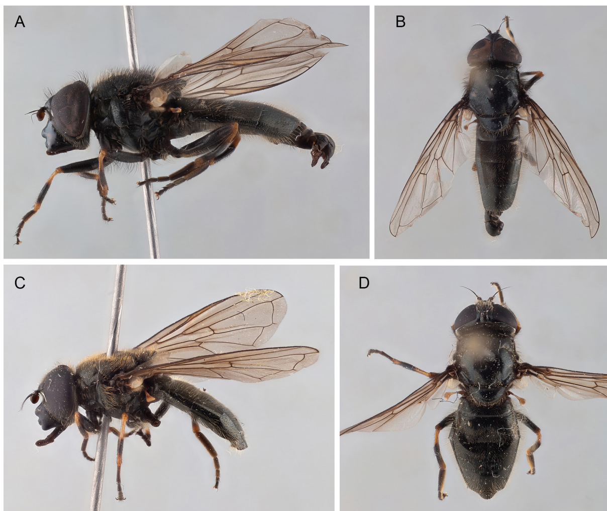
Fig. 21. Cheilosia (Cheilosia) confusa sp. nov. A–B. Holotype, ♂ (ZFMK, ZFMK-TIS-8028459); habitus, lateral and dorsal views; body length 9.5 mm. C. Paratype, ♀ (SBA, CNC databasing S Bot 927); habitus, lateral view; body length 8.2 mm. D. Paratype, ♀ (SBA, ZFMK-TIS-8027995); habitus, dorsal view; body length 8.4 mm. Not to scale.
