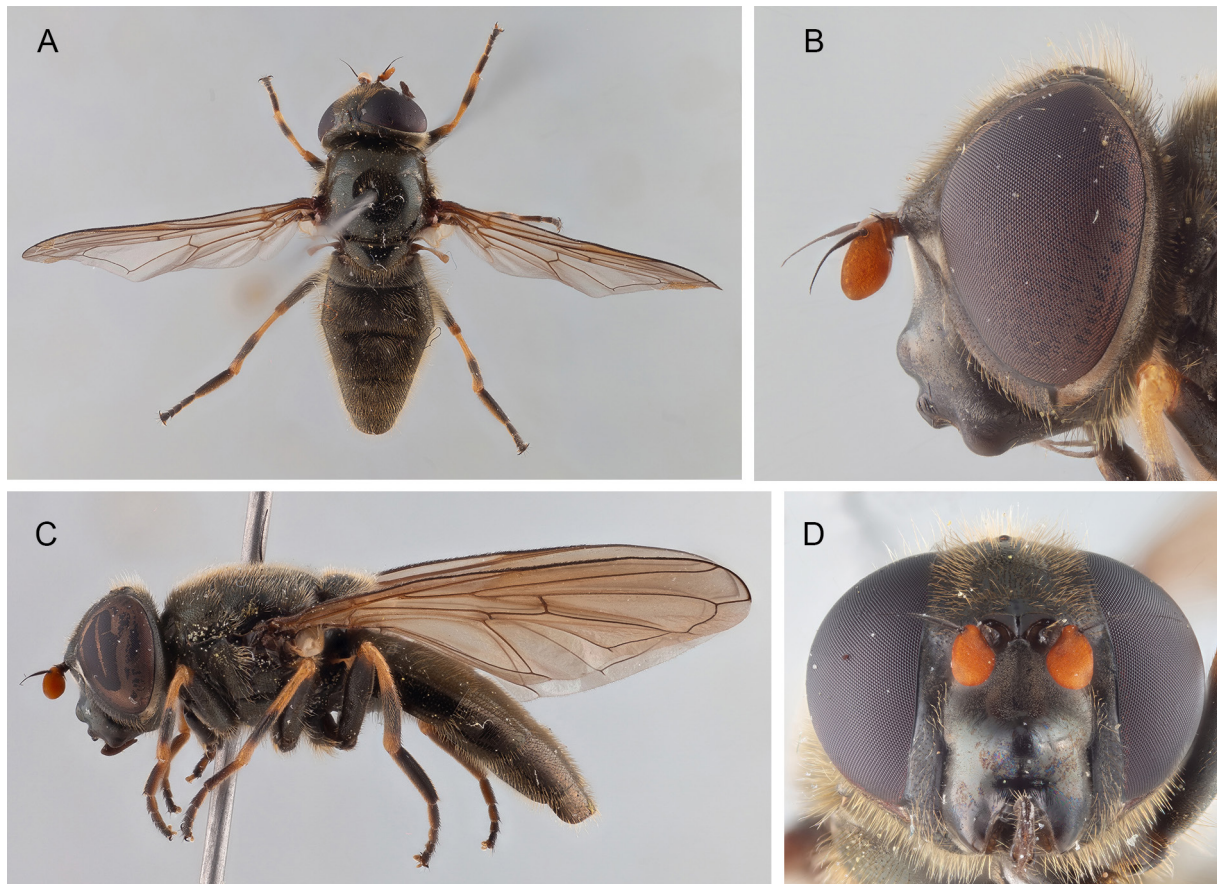
Fig. 45. Cheilosia (Cheilosia) megaclama sp. nov., ♀. A. Paratype (SBA, ZFMK-TIS-8027980); habitus, dorsal view; body length 8.8 mm. B. Paratype (FMT, ZFMK-TIS-8012674); head, lateral view; eye width 1.3 mm. C. Paratype (FMT); habitus, lateral view; body length 8.8 mm. D. Paratype (SBA, ZFMK-TIS-8027980); head, frontal view; head width 2.5 mm. Not to scale.
