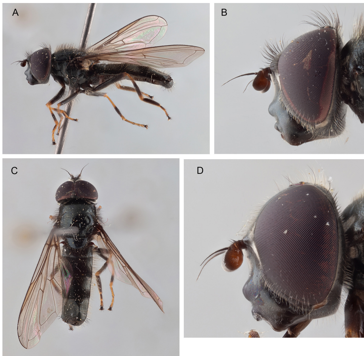
Fig. 71. Cheilosia (Cheilosia) urbana (Meigen, 1822). Collected in Georgia. A–C. ♂ (SBA, SB.002901. A. Habitus, lateral view; body length 6.8 mm. B. Head, lateral view; eye width 1.1 mm. C. Habitus, dorsal view; body length 6.8 mm. D. ♀ (SBA, SB.002919); head, lateral view; eye width 1.1 mm. Not to scale.
