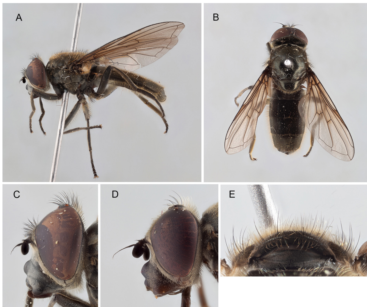
Fig. 2. Cheilosia (Taeniochilosia) aenigmatorosa Barkalov, 1993. Collected in Georgia. A. ♂ (SBA, SB.003064); habitus, lateral view; body length 8.3 mm. B. ♂ (SBA, SB.003064); habitus, dorsal view; body length 8.3 mm. C. ♂ (SBA, SB.003064); head, lateral view; eye width 1.1 mm. D. ♀ (SBA, SB.003063); head, lateral view; eye width 1.3 mm. E. ♂ (SBA, SB.003062); scutellum, posterior view; scutellum width 1.7 mm. Not to scale.
