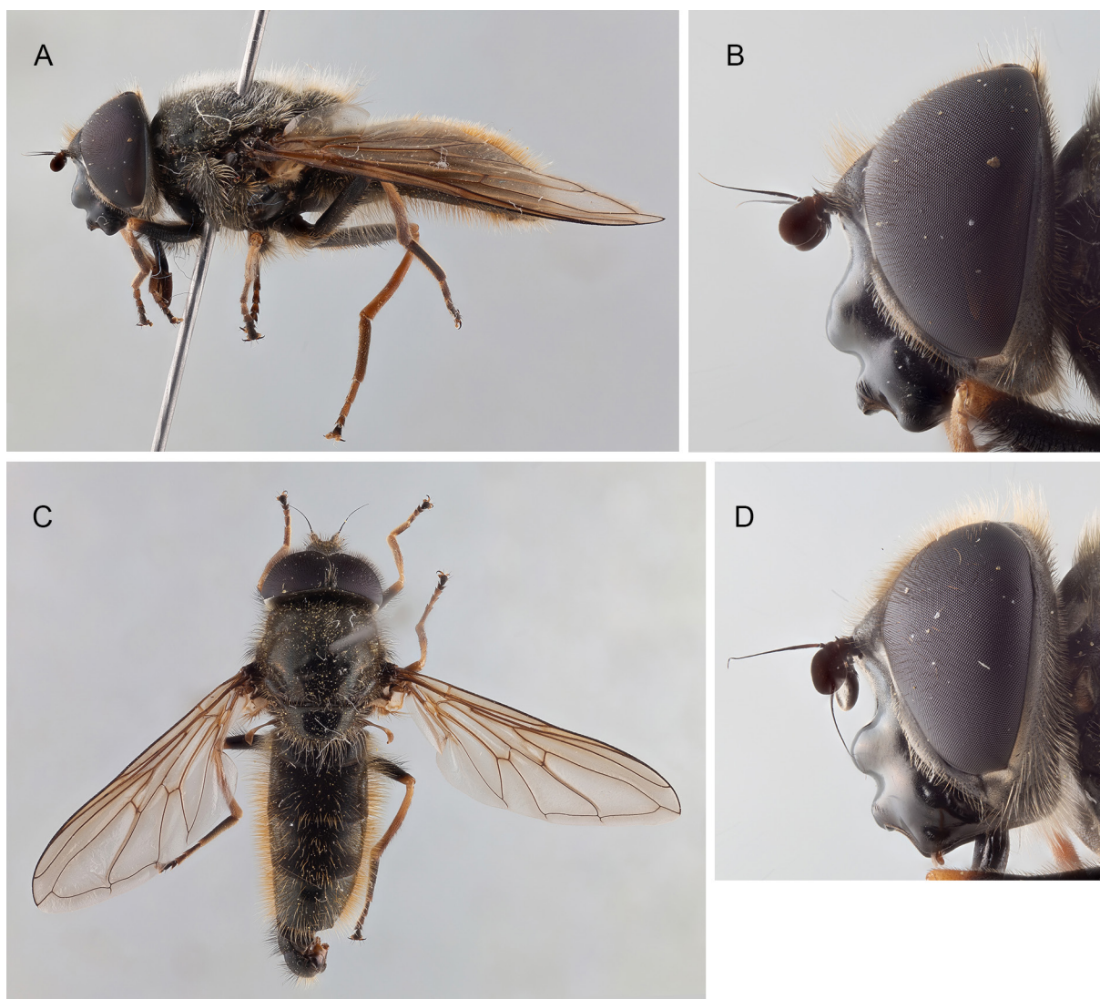
Fig. 50. Cheilosia (Cheilosia) orthotricha Vujić & Claussen, 1994. Collected in Georgia. A. ♂ (SBA, SB.002710); habitus, lateral view; body length 13.5 mm. B. ♂ (SBA, SB.002710); head, lateral view; eye width 1.6 mm. C. ♂ (SBA, ZFMK-TIS-8028450); habitus, dorsal view; body length 14.1 mm. D. ♀ (SBA, SB.002711); head, lateral view; eye width 1.5 mm. Not to scale.
