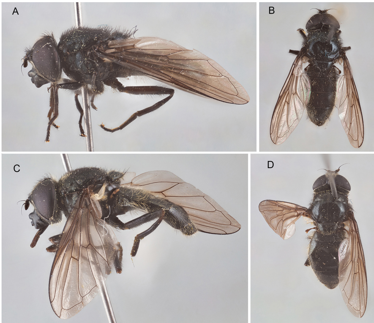
Fig. 18. Cheilosia (Cheilosia) caucasi sp. nov. A–B. Holotype, ♂ (ZFMK, ZFMK-DIP-00066397); habitus, lateral and dorsal views; body length 9.2 mm. C–D. Paratype, ♀ (ZFMK, ZFMK-DIP-00066398); habitus, lateral and dorsal views; body length 9.4 mm. Not to scale.
