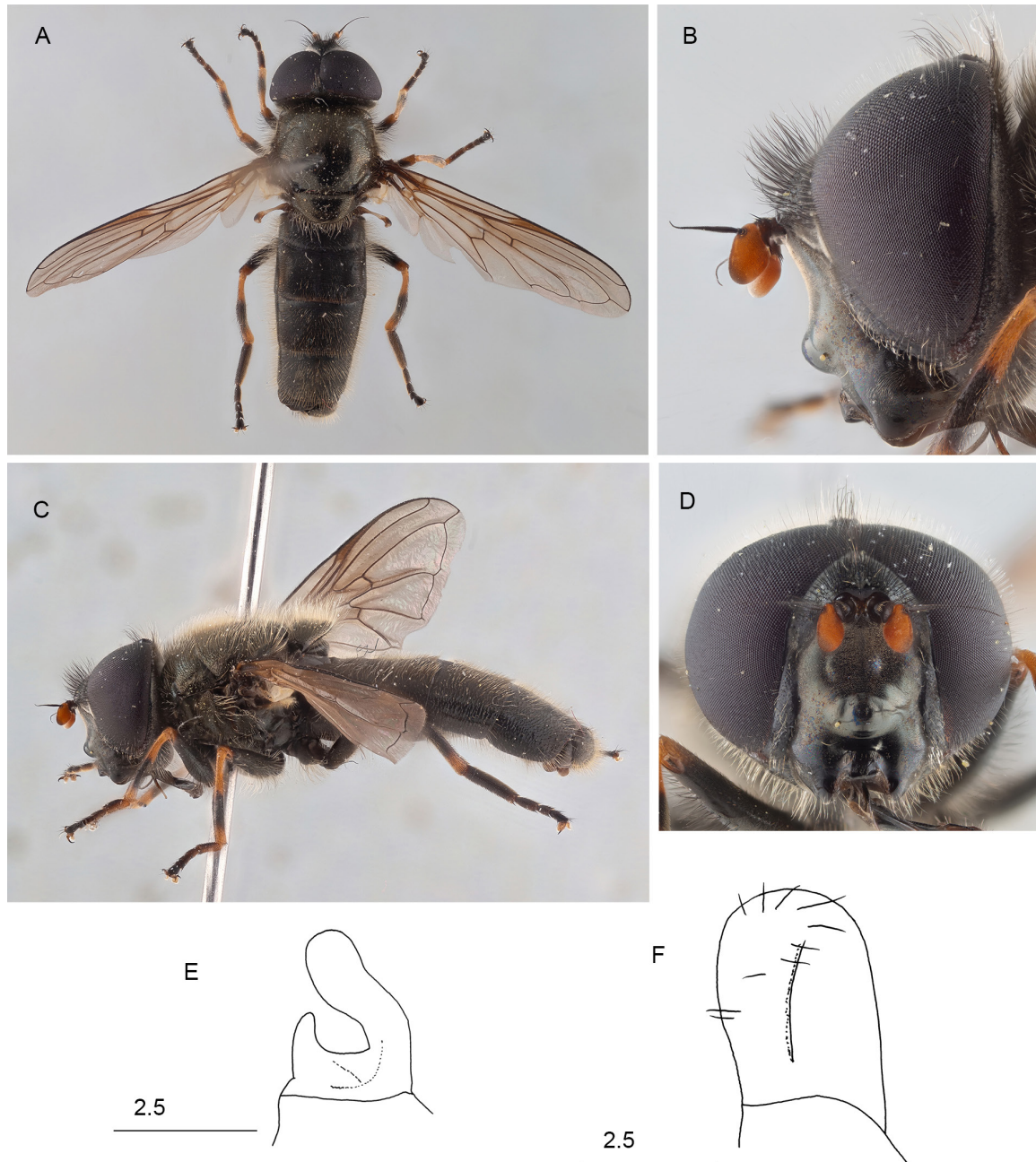
Fig. 44. Cheilosia (Cheilosia) megaclama sp. nov., paratype, ♂ (SBA, SB.003217); body length 10.5 mm. A. Habitus, dorsal view. B. Head, lateral view; eye width 1.4 mm. C. Habitus, lateral view. D. Head frontal view; head width 2.5 mm. E. Postgonite, lateral view. F. Surstylus, lateral view. Scale bars: A–D not to scale; E–F in \mu\text{m} .
