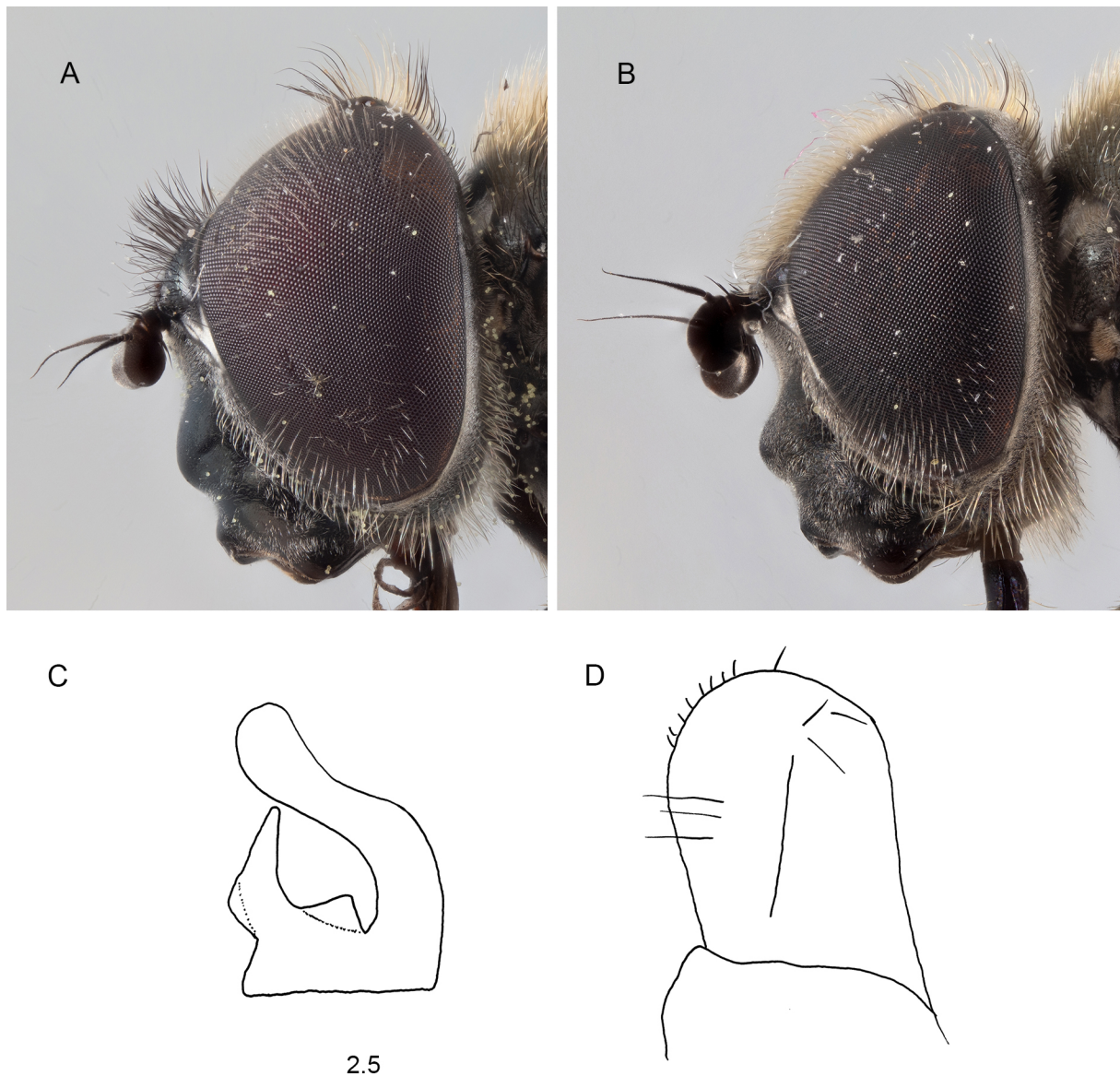
Fig. 73. Cheilosia (Cheilosia) ushguliensis sp. nov. A. Holotype, ♂ (ZFMK, ZFMK-DIP-00066503); head, lateral view; eye width 1.3 mm. B. Paratype, ♀ (ZFMK, ZFMK-DIP-00066608); head, lateral view; eye width 1.4 mm. C. Paratype, ♂ (SBA); postgonite, lateral view. D. Paratype, ♂ (SBA); surstylus, lateral view. Scale bar: A–B not to scale; C–D in \mu\text{m} .
