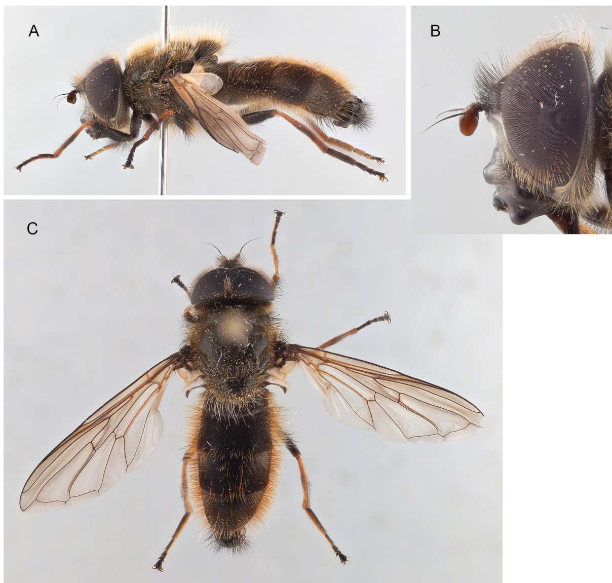
Fig. 58. Cheilosia (Cheilosia) pseudogrossa Stackelberg, 1968. Collected in Georgia. A. ♂ (SBA, ZFMK-TIS-8027992); habitus, lateral view; body length 13.4 mm. B. ♂ (FMT, ZFMK-TIS-8027940); head, lateral view; eye width 1.5 mm. C. ♂ (SBA, ZFMK-TIS-8027992); habitus, dorsal view; body length 13.4 mm. Not to scale.
