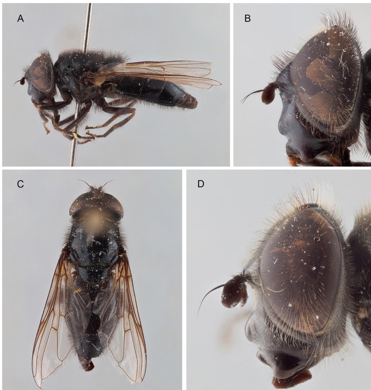
Fig. 11. Cheilosia ( Montanocheila ) balu Violovitsh, 1966. Collected in Georgia. A. ♂ (ZFMK, ZFMK-DIP-00058266); habitus, lateral view; body length 11.2 mm. B. ♂ (ZFMK, ZFMK-DIP-00058266); head, lateral view; eye width 1.3 mm. C. ♂ (ZFMK, ZFMK-DIP-00058266); habitus, dorsal view; body length 11.2 mm. D. ♀ (ZFMK, ZFMK-DIP-00058267); head, lateral view; eye width 1.3 mm. Not to scale.
