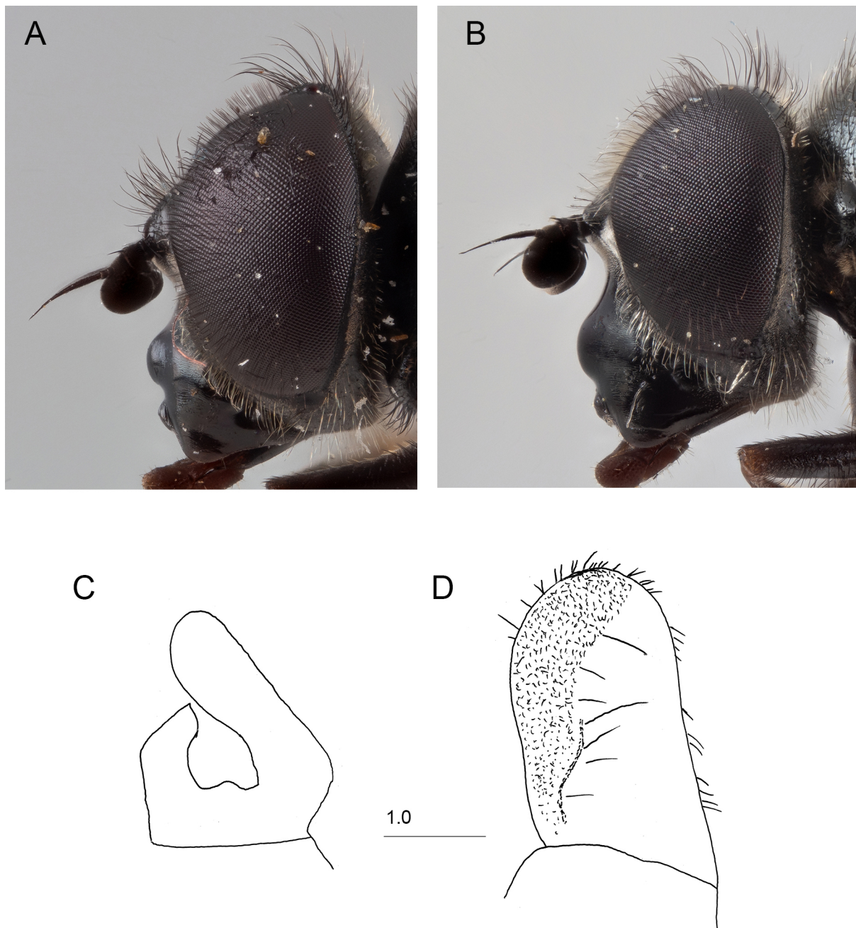
Fig. 30. Cheilosia (Cheilosia) gemmula sp. nov. A. Holotype, ♂ (ZFMK, ZFMK-TIS-8009652); head, lateral view; eye width 0.9 mm. B. Paratype, ♀ (SBA, ZFMK-TIS-8009653); head, lateral view; eye width 0.9 mm. C–D. Paratype, ♂ (SBA, SB.003133). C. Postgonite, lateral view. D. Surstylus, lateral view. Scale bars: A–B not to scale; C–D in \mu\text{m} .
