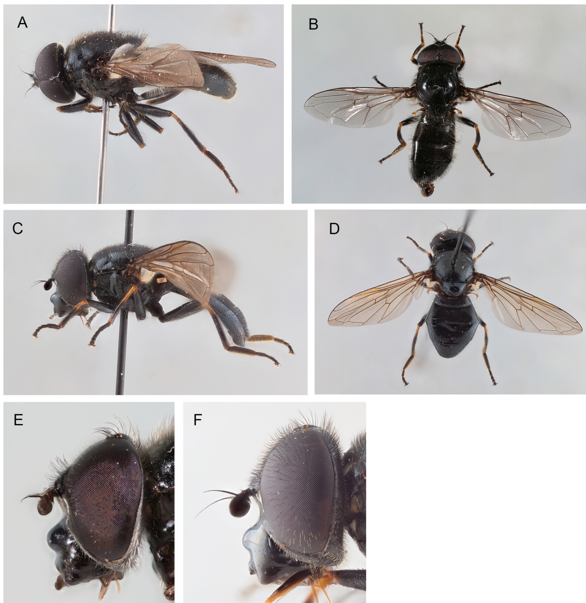
Fig. 26. Cheilosia (Cheilosia) cynocephala Loew, 1840. A. ♂ (SBA, SB.004468); habitus, lateral view; collected in Altai Republic, Russia; body length 9.9 mm. B. ♂ (FMT); habitus, dorsal view; collected in Belgium; body length 8.7 mm. C. ♀ (FMT); habitus, lateral view; collected in Georgia; body length 8.3 mm. D. ♀ (FMT); habitus, dorsal view; collected in Georgia; body length 8.3 mm. E. ♂ (FMB); head, lateral view; collected in Belgium; eye width 1.3 mm. F. ♀ (FMT); head, lateral view; collected in Georgia; eye width 1.2 mm. Not to scale.
