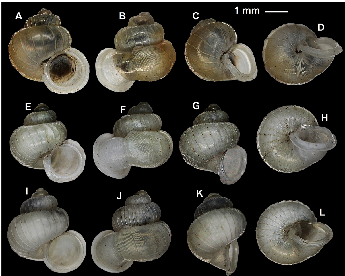
Fig. 24. Shells of species of Cycloryx Godwin-Austen, 1914 from Bhutan. A–D. C. globhutanus Gittenberger & Sherub Sherub, 2022, holotype (NBCB 1285). E–H. C. haumbiclausus Gittenberger & Choki Gyeltshen, 2022, holotype (NBCB 1272). I–L. C. sajumbiclausus Gittenberger & Choki Gyeltshen, 2022, holotype (NBCB 1290). All photos from Gittenberger et al. (2022).
