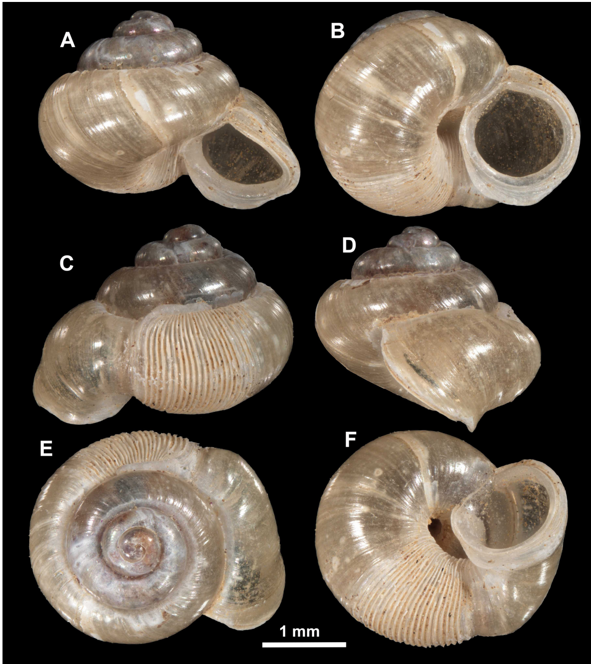
Fig. 57. Dicharax praeda Páll-Gergely & Aravind sp. nov., holotype (NZSI LM1740). All photos: B. Páll-Gergely.
