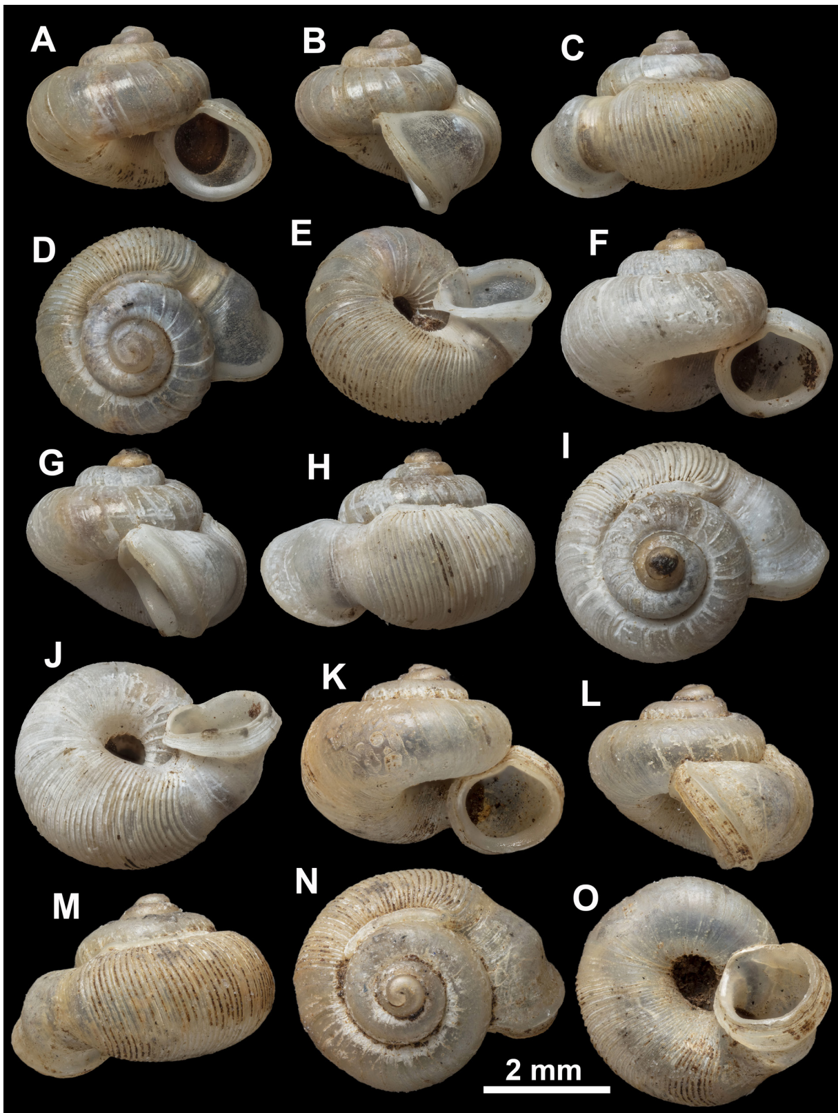
Fig. 69. Shells of Dicharax theobaldi (W.T. Blanford, 1862). A–E. Syntype of Alycaeus theobaldi (NHMUK 1906.4.4.60). F–J. Syntype of A. theobaldi var. diyungensis (NHMUK 1903.7.1.2546). K–O. Syntype of A. maosmaiensis (NHMUK 20191067). All photos: Kevin Webb.
