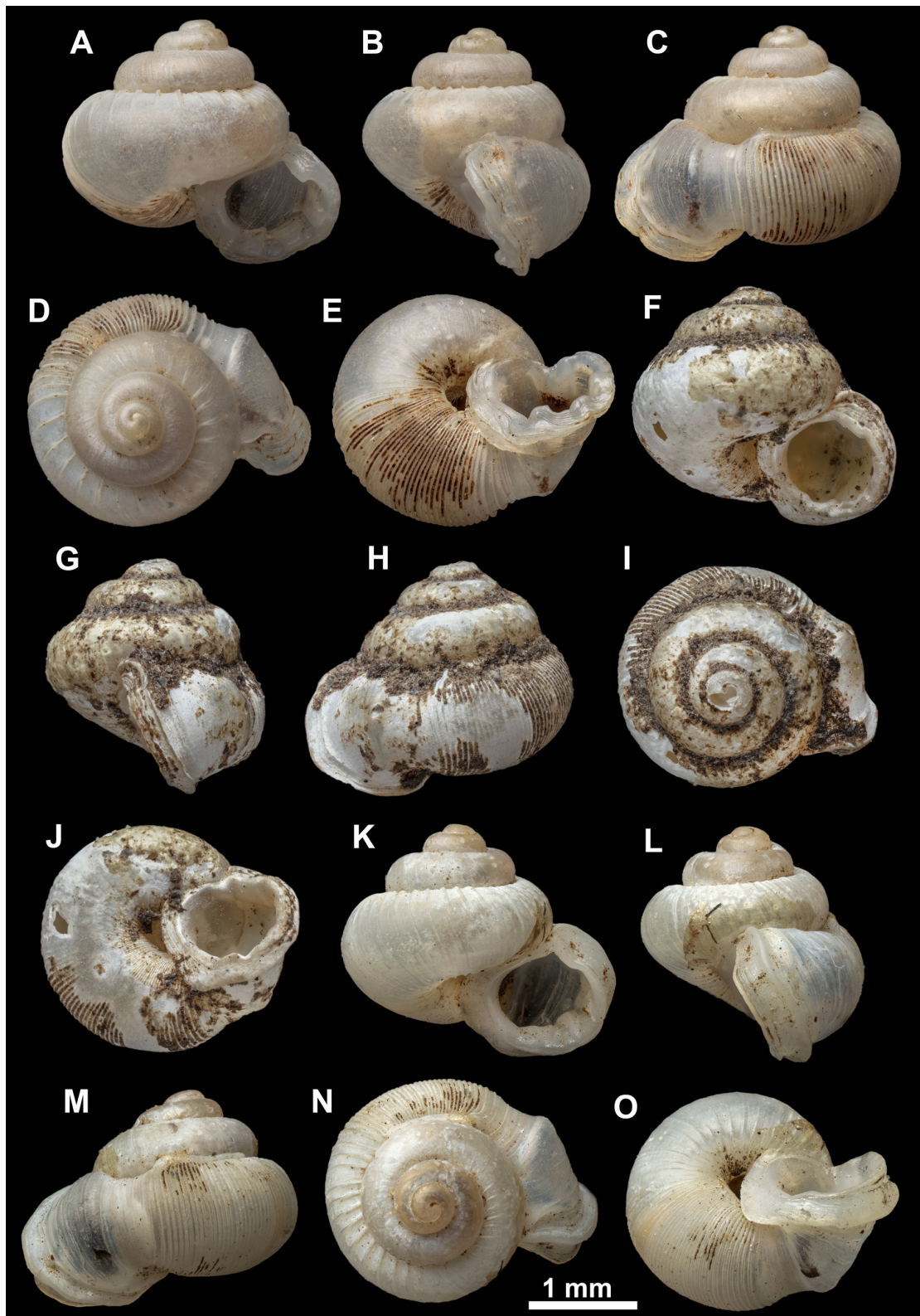
Fig. 32. Shells of Dicharax jaintiacus (Godwin-Austen, 1871). A–E. Syntype of Alycaeus jaintiacus Godwin-Austen, 1871 (NHMUK 1903.7.1.2686). F–J. Syntype of A. serratus Godwin-Austen, 1874 (NHMUK 1903.7.1.2487). K–O. Syntype of A. jaintiacus var. crassus Godwin-Austen, 1914 (NHMUK 1903.7.1.2752). All photos: Kevin Webb.
