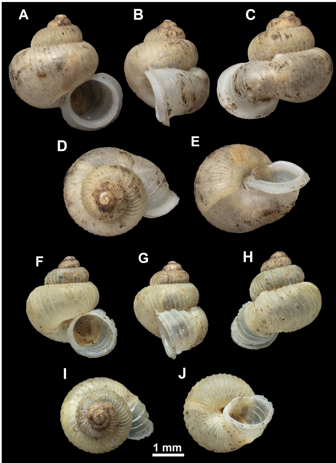
Fig. 23. Shells of species of Cyclorhynchus Godwin-Austen, 1914. A–E. C. dihingensis (Godwin-Austen, 1914), syntype (NHMUK 1903.7.1.2516). F–J. C. paucicostatus (Godwin-Austen, 1914), syntype (NHMUK 1903.7.1.2595). All photos: Kevin Webb.
