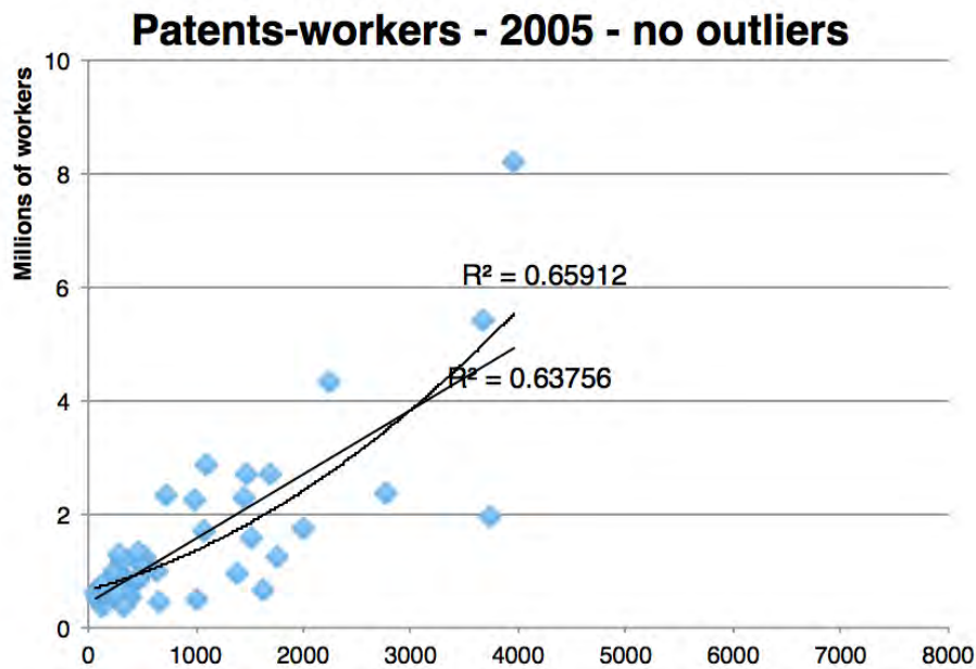
Figure 6. Linear and polynomial regression without two outliers.
