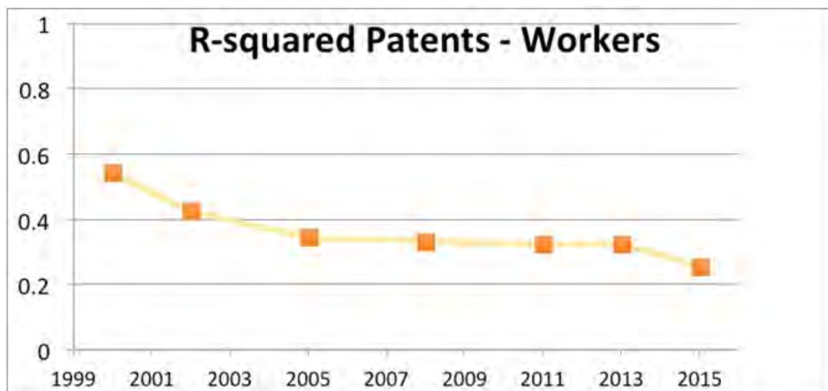
Figure 2. Coefficient of determination (R-squared) Patents-Workers for US metro areas from 2000-2015
