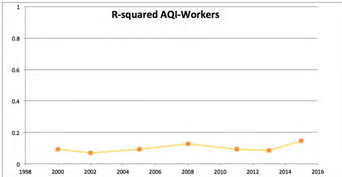
Figure 4. R-squared between AQI-Workers for the US metro areas in the period 2000-2015
