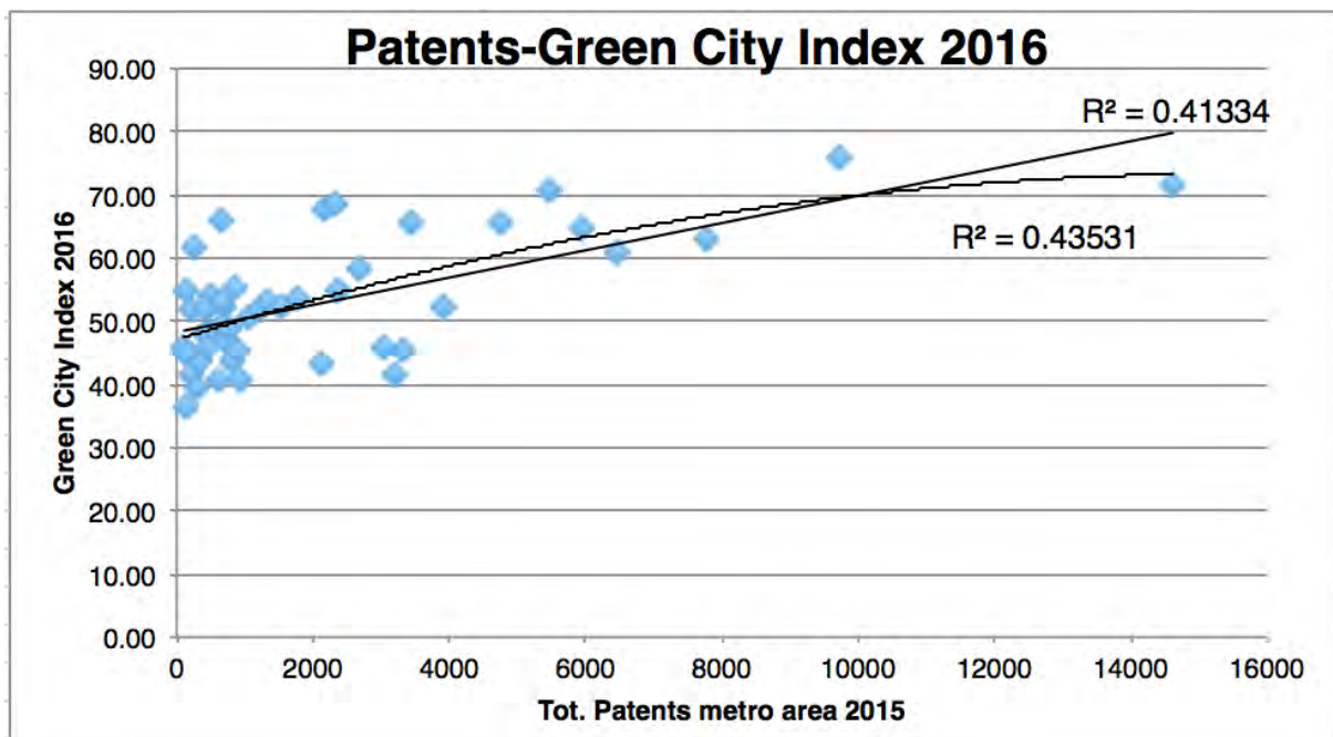
Figure 7. Regression between Patents and Green City Index for US metro areas
