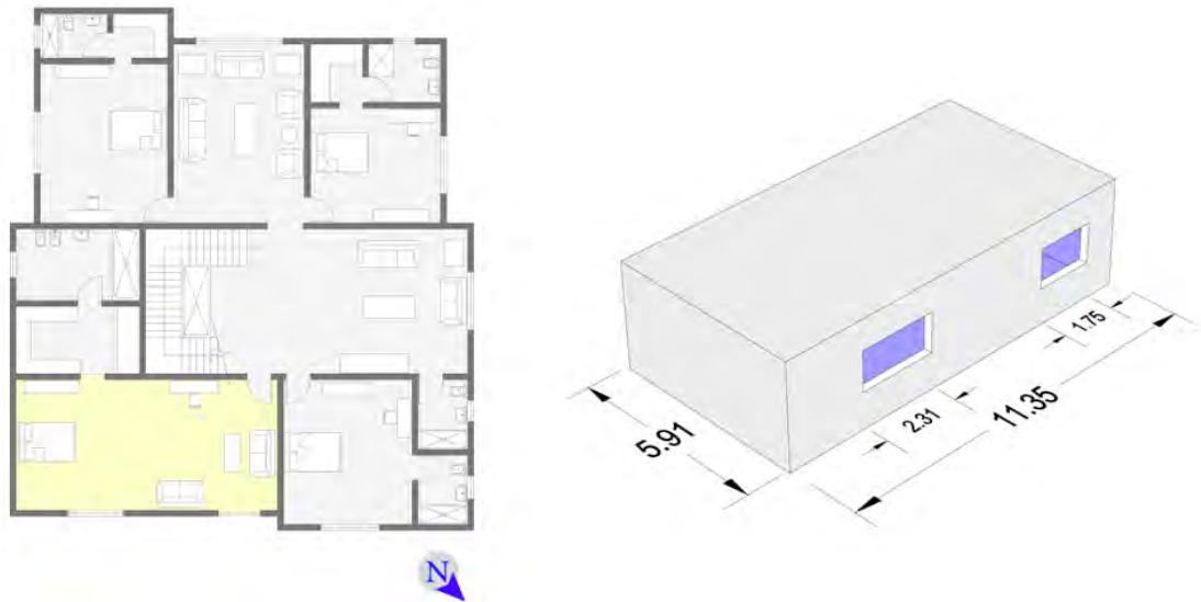
Figure 5. Layout of the residential unit and the master bedroom marked in yellow (left), the geometric model for the master bedroom (right)
