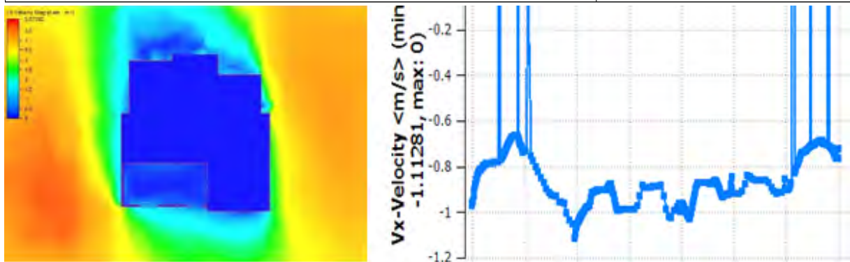
Figure 6. The air flow distribution outside and inside the master bedroom (left), the V_x velocity normal to the inlet window (right)
