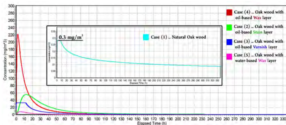
Figure 7. The analysis of TVOC concentrations of the Cases v.s elapsed time
