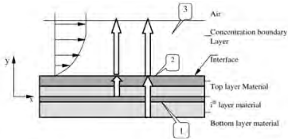
Figure 2. Physical configuration of VOC emissions from a multi-layer material. (1) Internal diffusion; (2) desorption; and (3) external convection and diffusion (Haghighat & Huang, 2003).
