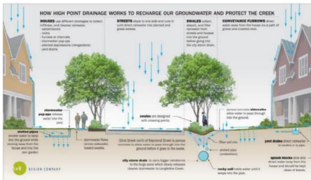
Figure 09: Drainage Diagram. Seattle High Point Community
