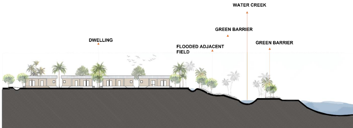
Fig 28. The riverside land should have two layers of green barrier with an agricultural buffer to reduce land loss and to trap the water at different levels
