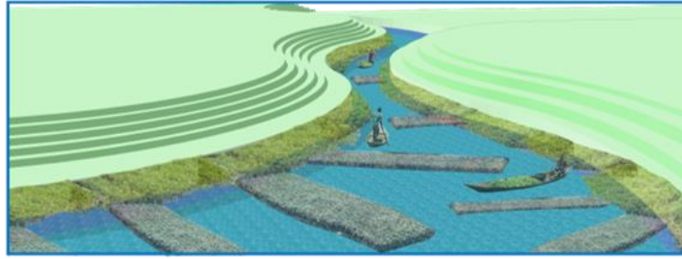
Fig 22. The proposed wetland with a floating garden in the rainy season
