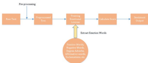
Figure 3: Flow Chart of Sentiment Analysis Method Based on Sentiment Dictionary
