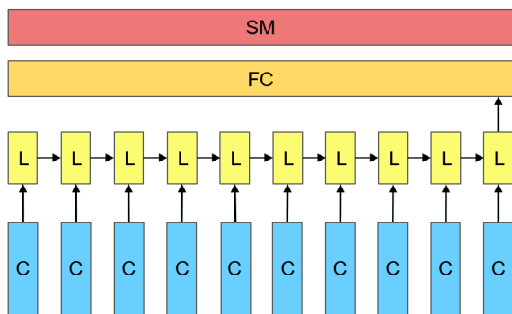
Figure 7. Long Short-Term Memory Networks
