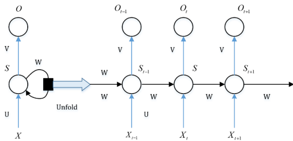
Figure 6. Recurrent Neural Networks
