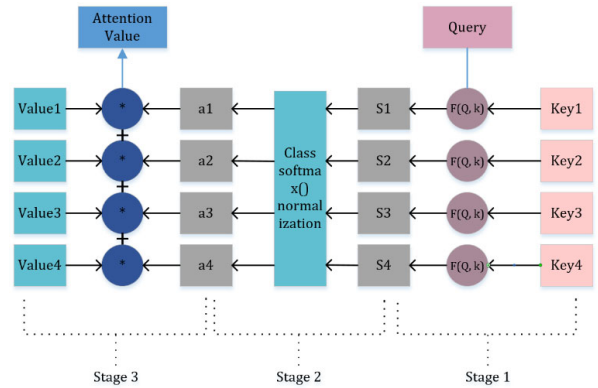
Figure 8. Attention Mechanism Module
