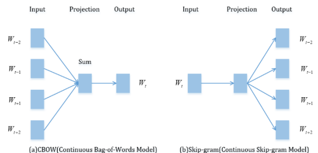
Figure 2. CBOW and Skip-gram Models
