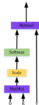
Figure 9. Self-Attention Mechanism Module
