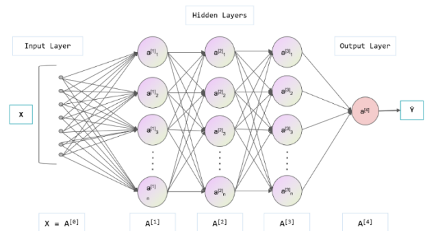
Figure 4. Neural Network Model
