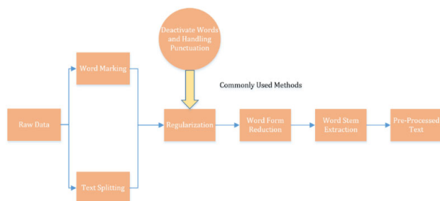
Figure 1. Data Pre-processing Flow Chart
