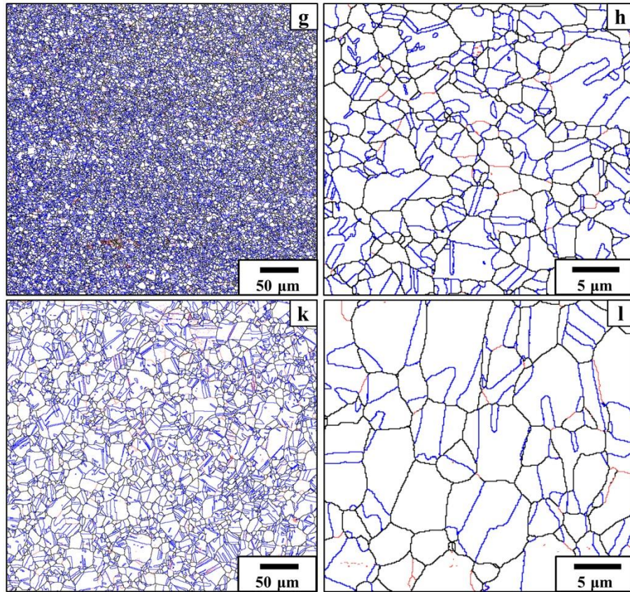
Fig. 2 (continuation) Grain boundary maps for Cu after CR and HDEP with current density of 6.8 \times 10^4 (g,h) and 8.1 \times 10^4 A^2s/mm^4 (k,l). Scanning step 500 (g,k) and 100 nm (h,l)
