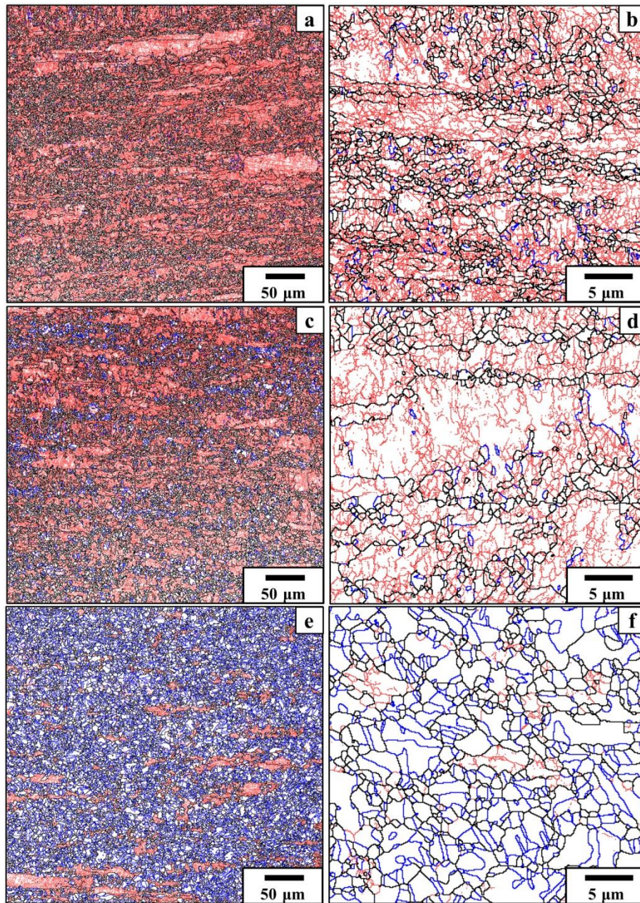
Fig. 2 Grain boundary maps for Cu after CR (a,b) and HDEP with current density of 3.5 \times 10^4 (c,d) and 3.8 \times 10^4 A 2 s/mm 4 (e,f). Scanning steps are 500 (a,c,e) and 100 nm (b,d,f). Hereafter red, black and blue lines indicate low-angle, high-angle and twin ( \Sigma 3 ) boundaries, consequently
