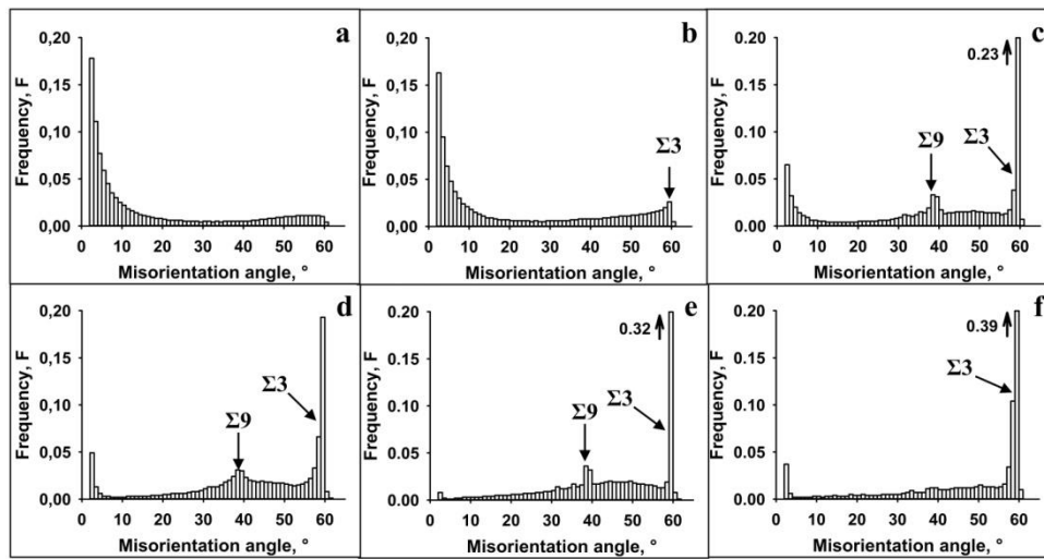
Fig. 3 Boundary spectra in Cu after CR (a) and HDEP with the current density of 3.5 \times 10^4 (b), 3.8 \times 10^4 (c), 5.0 \times 10^4 (d), 6.8 \times 10^4 (e) and 8.1 \times 10^4 \text{ A}^2/\text{mm}^4 (f). Scanning step is 500 nm.
