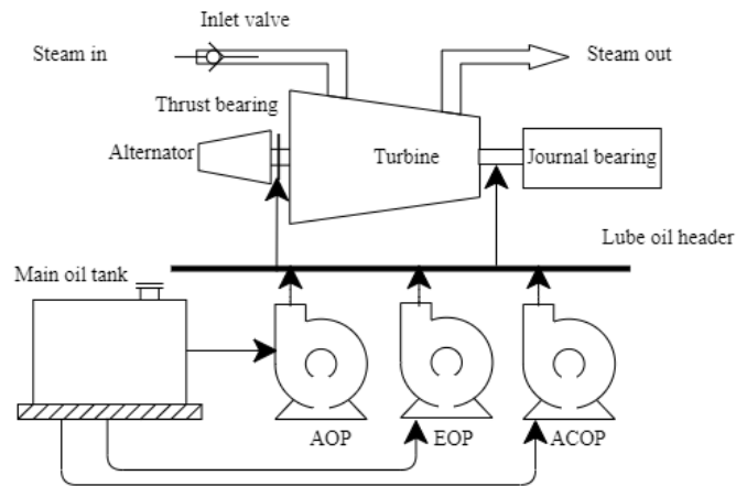
Fig. 2 Schematic arrangement of TAU
