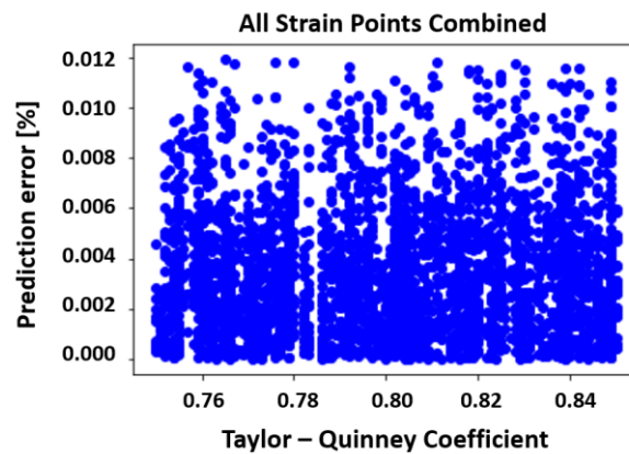
Fig. 11 Prediction error for the given TQC interval of all 12 points of the temperature increase curve – actual TQC ( \beta ) for the last strain point is shown
