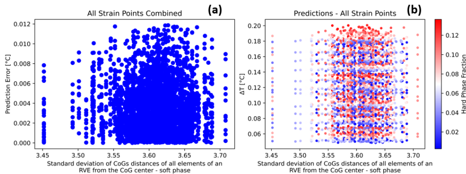
Fig. 16 Standard deviation of center of gravity distances of all elements of an RVE from the center of gravity center for all RVEs of all 12 points of the temperature increase curve – soft phase: (a) with prediction error and (b) with temperature increase
