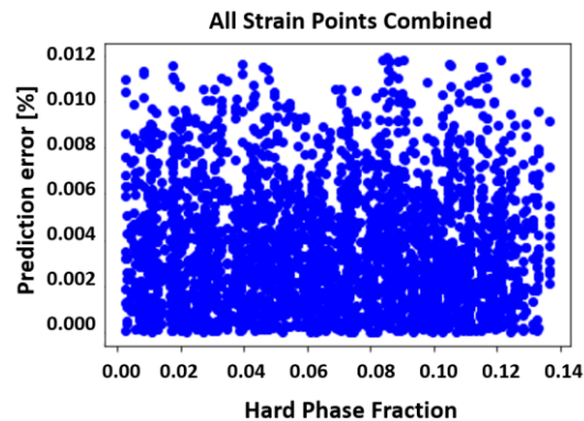
Fig. 13 Prediction error for the hard phase fraction interval of all 12 points of the temperature increase curve
