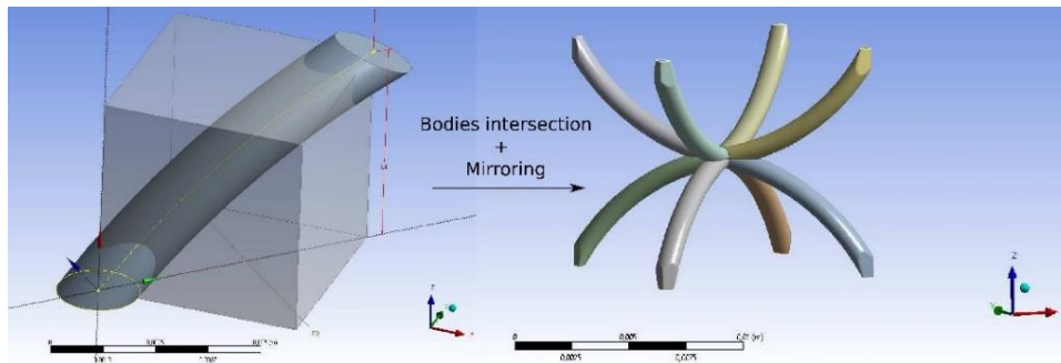
Fig. 2 BCC cell geometry definition, waved struts based on circumferential arch path
