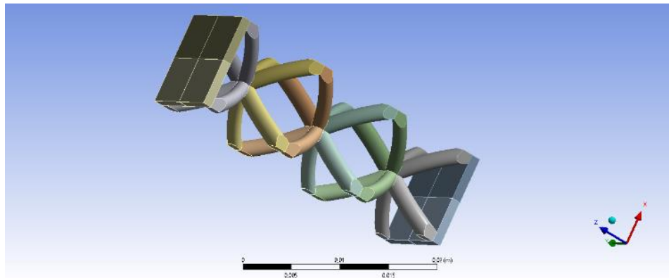
Fig. 17 Sandwich panel section made of structural steel skins and lattice core based on three waved BCC cells along the thickness direction
