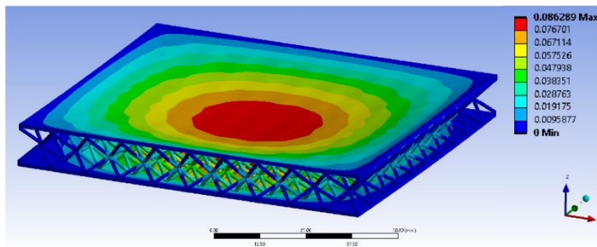
Fig. 10 Total displacement of the sandwich plate with lattice core made of 10 \times 10 pattern BCC cells with straight struts
