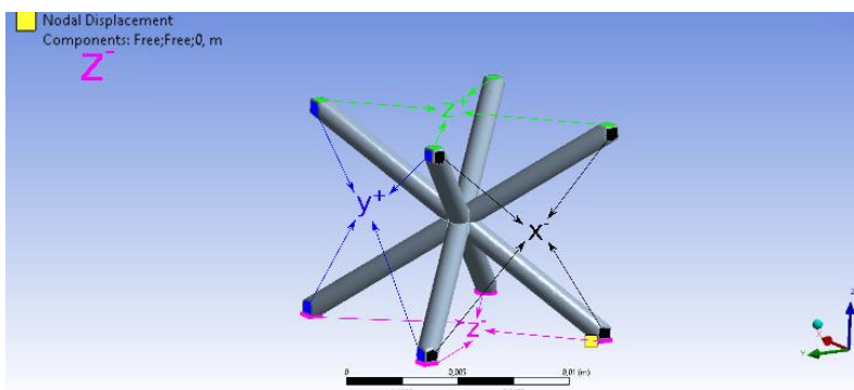
Fig. 3 BCC cell with straight struts, boundary definition
