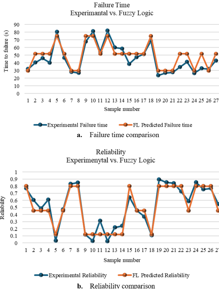
Fig. 6 Comparisons of failure time reliability values with their corresponding FL predicted values
