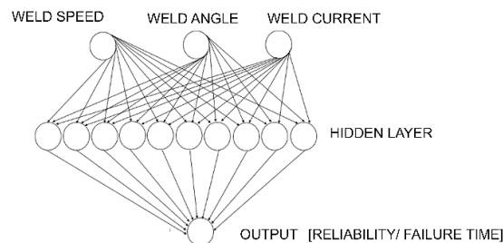
Fig. 4 Proposed structure of the ANN
