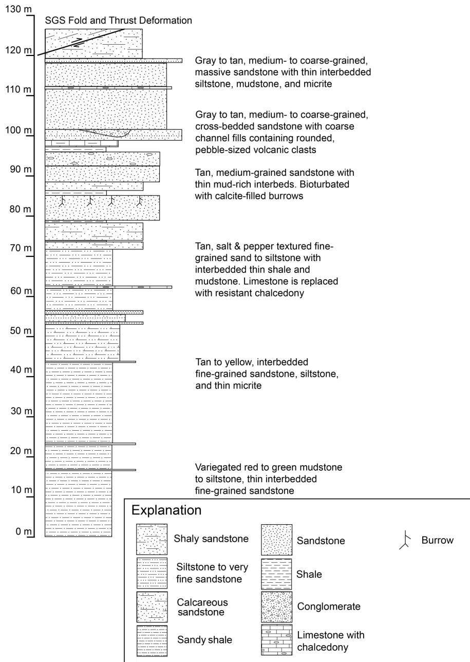
Figure 3. Stratigraphic column of the Brian Head Formation at the base of Casto Butte. Here the Brian Head is well exposed and approximately 125 m thick. The Brian Head Formation here rests disconformably over the Claron Formation, and it is overlain by allochthonous volcanic rocks of the Sevier gravity slide (SGS). The lower Brian Head consists of evenly stratified variegated mudstone, siltstone, and sandstone. The upper Brian Head is coarser grained, and consists of lithic wacke and arenite, conglomerate, and some limestone. The uppermost Brian Head was deformed by the emplacement of the SGS, some of it being incorporated into the slide basal layer (Mayback et al., 2022; Braunagel et al., 2025). We collected samples for the lower plate Casto and Blind Springs, and the uppermost Brian Head sandstone. For the upper plate Haycock sample, the collection horizon is uncertain.
