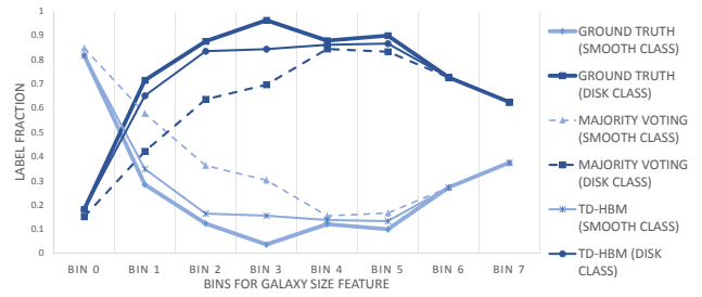
Figure 4: Label fractions for two most likely classes as a function of galaxy size. The figure displays ground truth fractions (thick line), predictions by majority voting (dashed line), and by TD-HBM (thin line).
