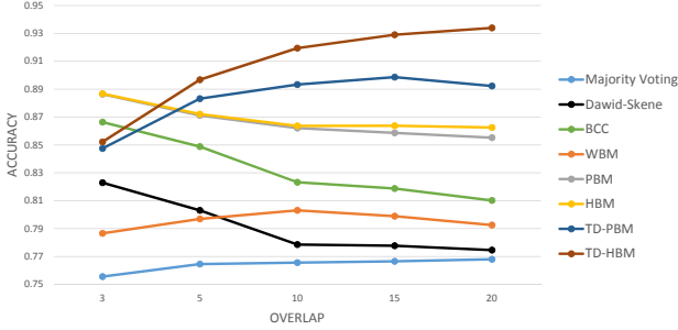
Figure 3: Accuracy of bias models with variation in annotation overlap.
