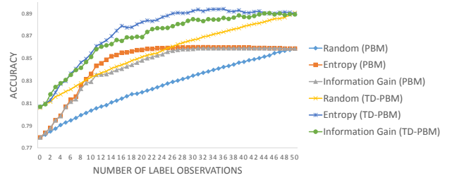
Figure 6: Accuracy of active learning methods.
