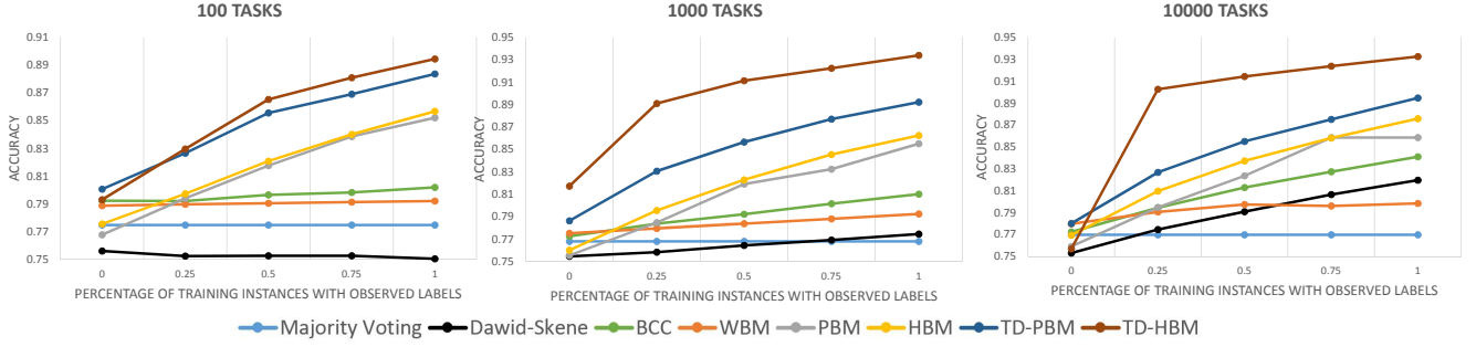
Figure 2: Accuracy of bias models with increasing number of ground truth label observations. The plots from left to right are for experiments with 100, 1000, and 10000 tasks respectively.
