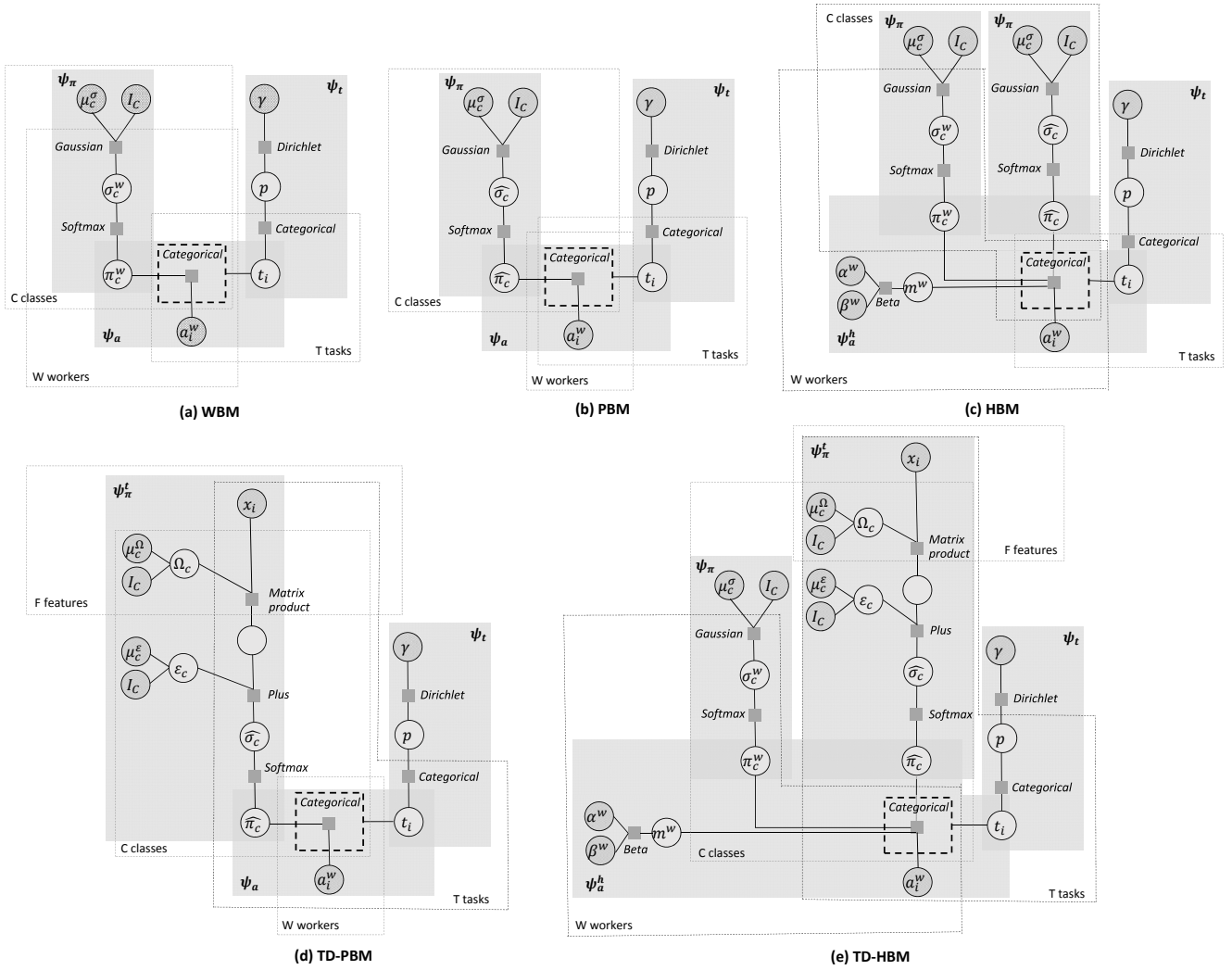
Figure 1: Models for representing and inferring bias. In each model, shaded regions mark potentials defined for inference. Dashed lines represent plates for classes, workers, and tasks. Gates are represented with darker dashed squares and observed variables are represented with shaded circles.
