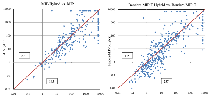
Figure 5: Run-time of Heuristic-Complete Approaches vs. Complete Approaches.
