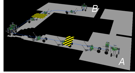
Figure 5: Roll-out of solution shown in Figure 4(c).
