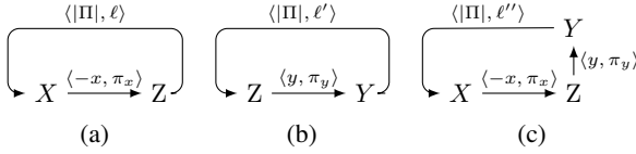
Figure 3: Paths discussed in the proof of Theorem 2
