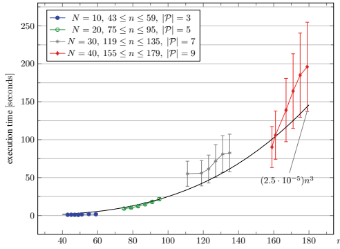
Figure 4: Execution time vs. number of time-points n
