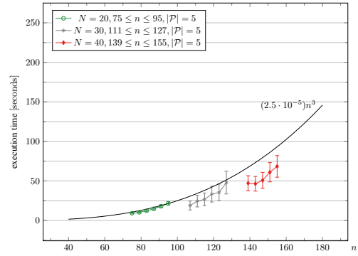
Figure 5: Execution time vs. number of time-points n . Number of proposition is constant.
