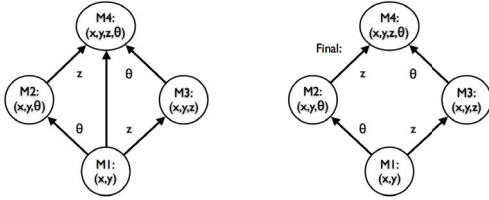
Figure 1: Transitive Reduction of original model graph.
