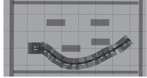
(b) Example XY\theta VA : notice that this higher model chooses to plan around the gurneys.
