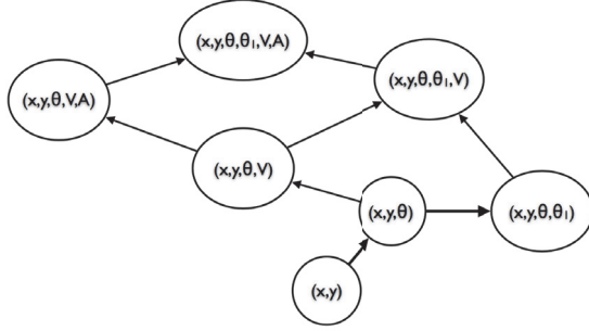
Figure 3: Transitive reduction of full model graph.
