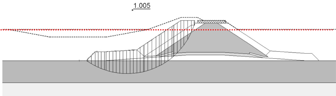
Figure 12. Modeling wave action in GEOSLOPE
