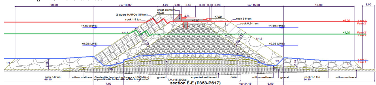
Figure 13. Construction phases of the Western breakwater
