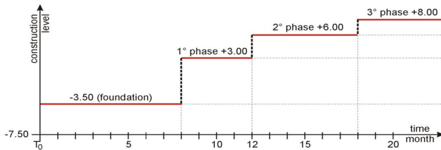
Figure 14. Construction steps in time.
