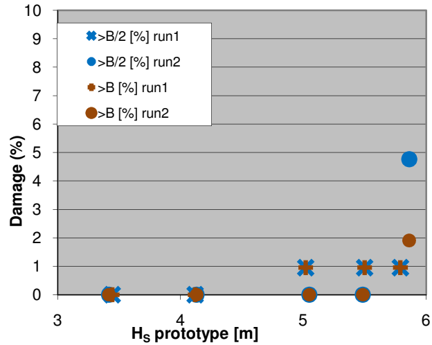
Figure 7. Damage graph of the double layer HAROs under increasing wave impact.
