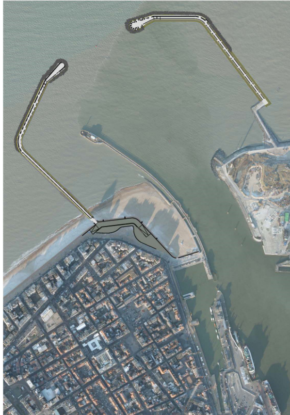
Figure 2. Renewed harbour entrance, protected by the Eastern and Western breakwaters (to be finished by august 2012)
