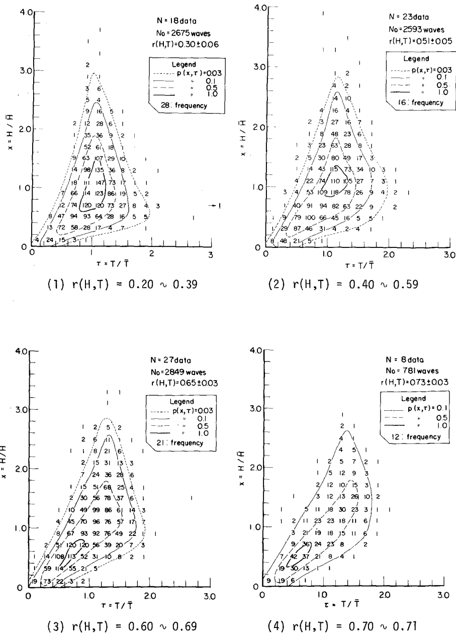
Fig. 7 Joint Distribution of Observed Wave Heights and Periods Grouped in the Rank of Correlation Coefficient, r(H, T)
