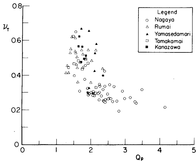
Fig. 14 Correlation between \nu_T and Q_p
