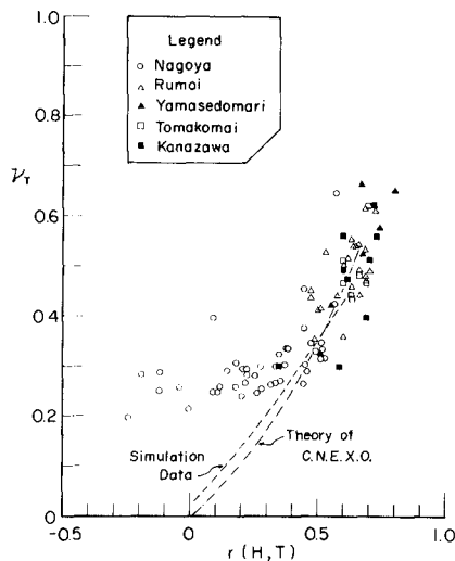
Fig. 10 Correlation between \nu_T and R(H,T)
