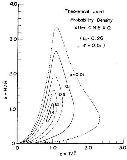
Fig. 2 Joint Probability Density by the Theory of C.N.E.X.O. ( \epsilon = 0.51 and \nu = 0.26 )
