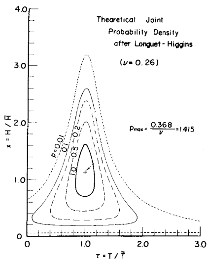
Fig. 1 Joint Probability Density by Longuet-Higgins' Theory ( \nu = 0.26 )
