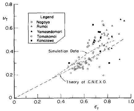
Fig. 12 Correlation between \nu_T and \epsilon_T
